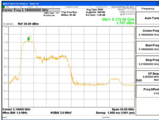
ANTO_802.11ax_HE40_52T_Low_UNI 1
