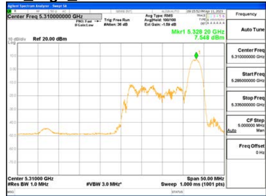
ANT1_802.11ax_HE40_26T_High_UNI 1A
