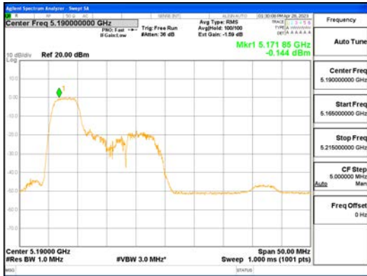
ANT1_802.11ax_HE40_52T_Low_UNI 1
