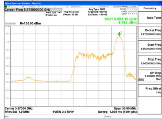
ANT1_802.11ax_HE40_26T_High_UNI 4
