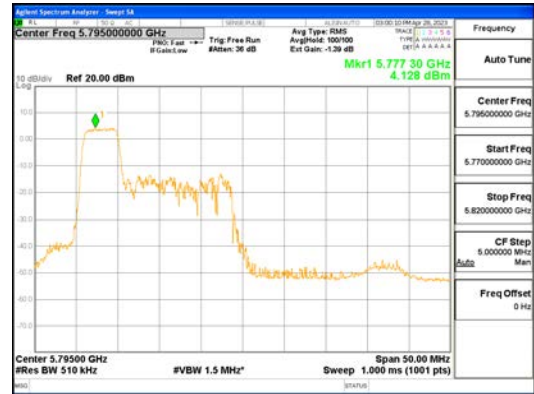
ANTO_802.11ax_HE40_52T_Low_UNI 3
