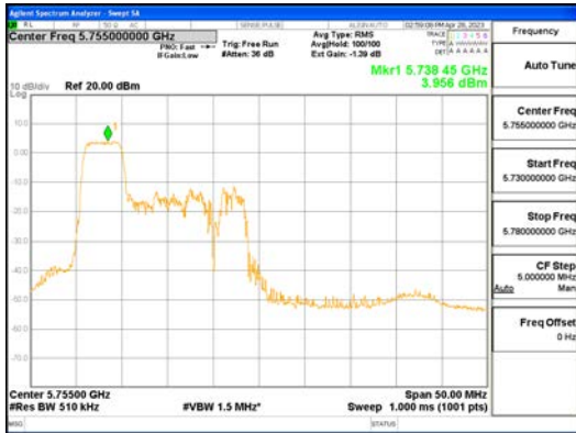
ANTO_802.11ax_HE40_52T_Low_UNI 3
