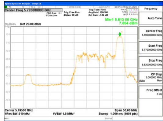
ANTO_802.11ax_HE40_26T_High_UNI I 3
