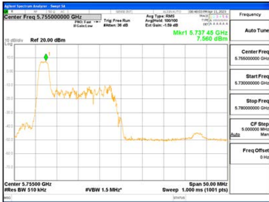
ANT1_802.11ax_HE40_26T_Low_UNI 3
