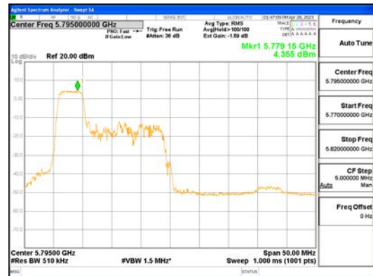
ANT1_802.11ax_HE40_52T_Low_UNI 3
