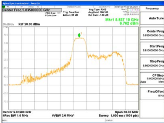
ANTO_802.11ax_HE40_52T_Mid_UNI I 4
