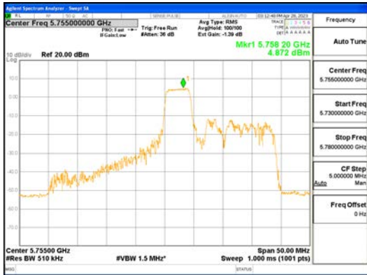
ANTO_802.11ax_HE40_52T_Mid_UNI I 3
