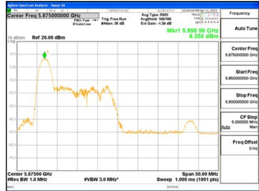
ANTO_802.11ax_HE40_26T_Low_UNI 4
