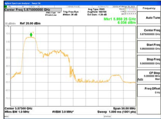
ANTO_802.11ax_HE40_52T_Low_UNI 4
