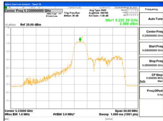
ANTO_802.11ax_HE40_52T_Mid_UNII 1
