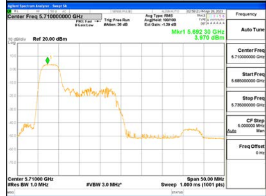
ANTO_802.11ax_HE40_52T_Low_UNI 2C
