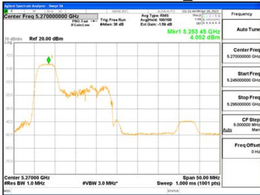
ANT1_802.11ax_HE40_52T_Low_UNI 2A
