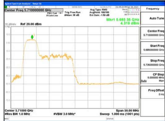
ANT1_802.11ax_HE40_52T_Low_UNI 2C
