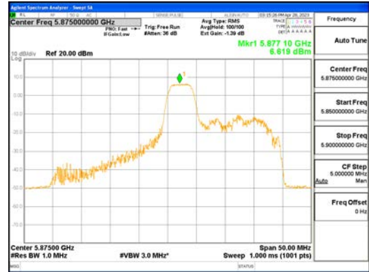
ANTO_802.11ax_HE40_52T_Mid_UNI I 4
