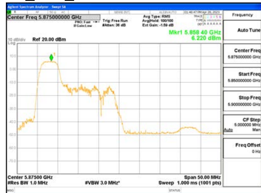
ANT1_802.11ax_HE40_52T_Low_UNI 4
