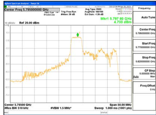
ANTO_802.11ax_HE40_52T_Mid_UNI I 3
