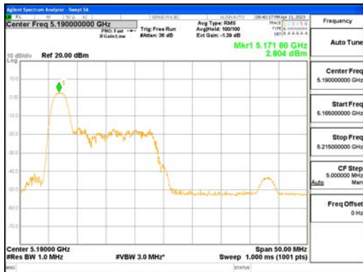
ANTO_802.11ax_HE40_26T_Low_UNI 1
