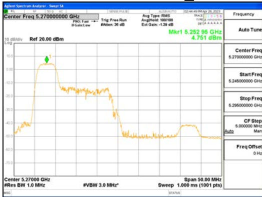
ANTO_802.11ax_HE40_52T_Low_UNI 2A
