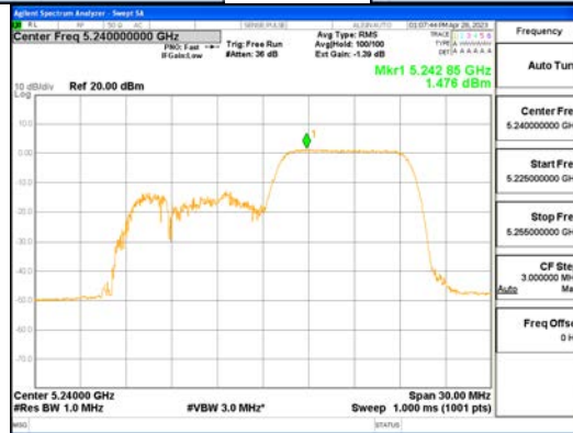
ANTO_802.11ax_HE20_106T_High_UNII 1
