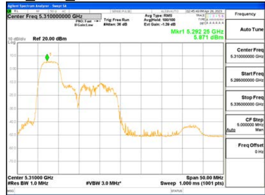
ANTO_802.11ax_HE40_52T_Low_UNI 2A
