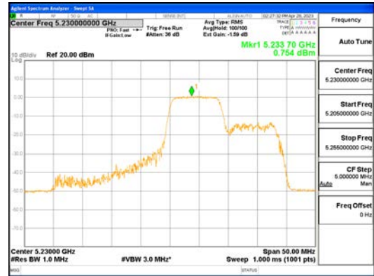
ANT1_802.11ax_HE40_106T_Mid_UNI 1
