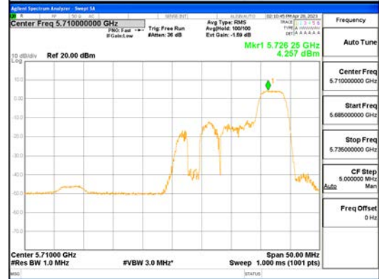
ANT1_802.11ax_HE40_52T_High_UNI 1C
