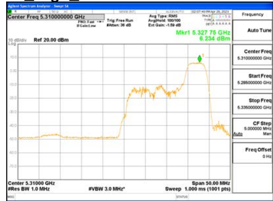
ANT1_802.11ax_HE40_52T_High_UNI 1A
