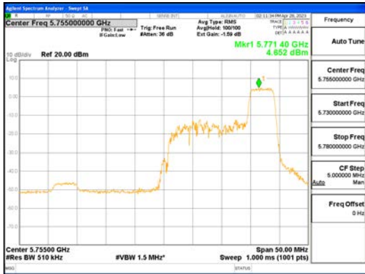
ANT1_802.11ax_HE40_52T_High_UNI 3
