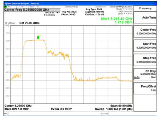
ANTO_802.11ax_HE40_106T_Low_UNII 1
