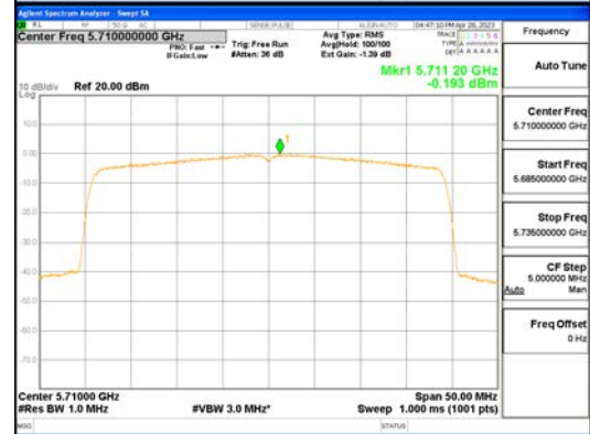
ANTO_802.11ax_HE40_484T_UNI 2C
