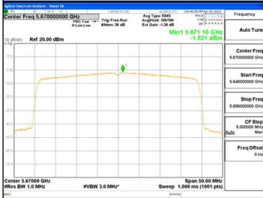
ANTO_802.11ax_HE40_484T_UNI 2C
