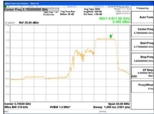
ANTI_802.11ax_HE40_106T_High_UNI I 3
