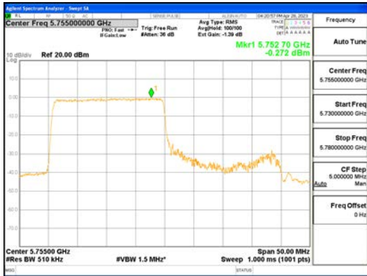
ANTO_802.11ax_HE40_242T_Low_UNI I 3
