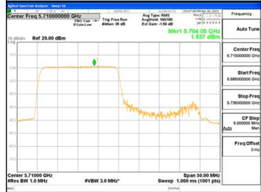
ANT1_802.11ax_HE40_242T_Low_UNII 2C
