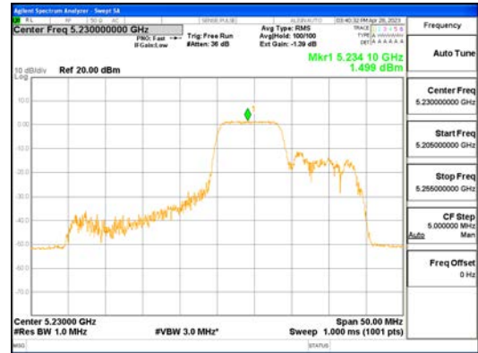
ANTO_802.11ax_HE40_106T_Mid_UNI I 1
