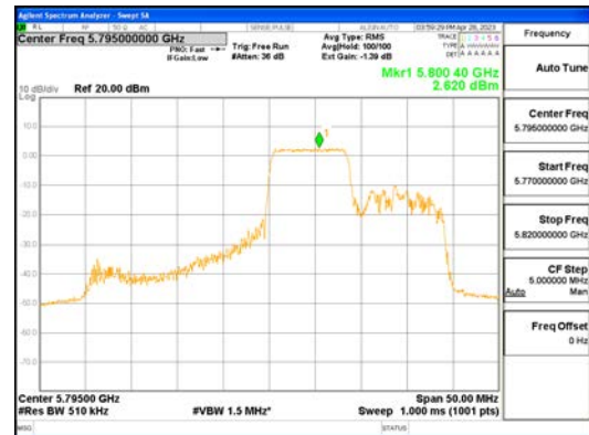
ANTO_802.11ax_HE40_106T_Mid_UNI I 3
