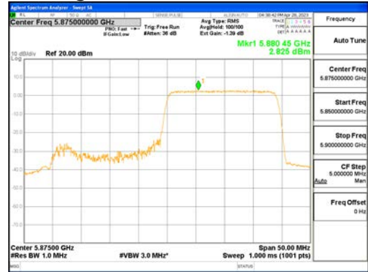
ANTO_802.11ax_HE40_242T_High_UNI I 4
