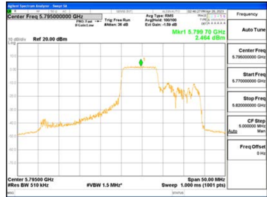
ANT1_802.11ax_HE40_106T_Mid_UNI I 3
