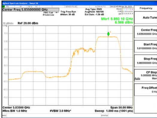
ANTO_802.11ax_HE40_106T_High_UNI I 4
