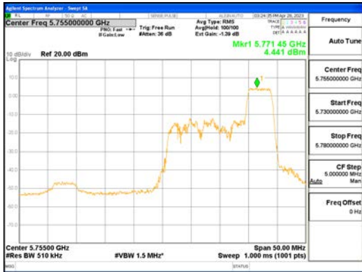
ANTO_802.11ax_HE40_52T_High_UNI 3
