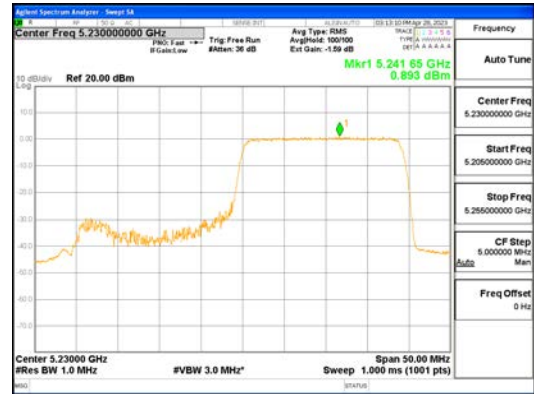
ANT1_802.11ax_HE40_242T_High_UNI I 1
