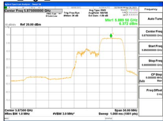
ANTI_802.11ax_HE40_106T_High_UNI I 4
