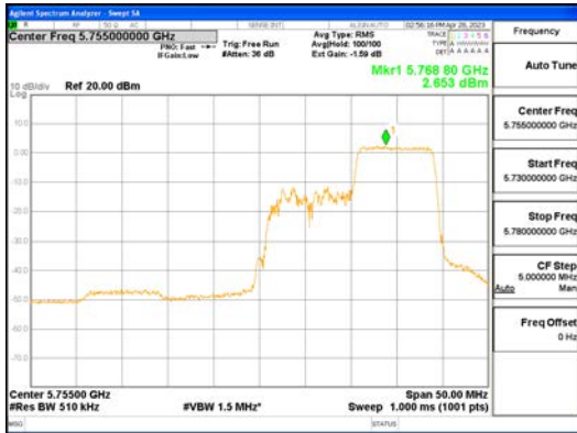
ANTI_802.11ax_HE40_106T_High_UNI I 3
