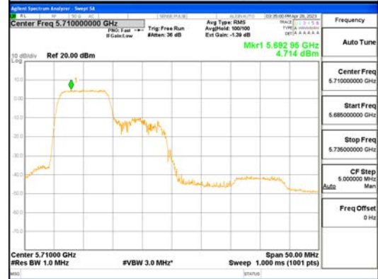
ANTO_802.11ax_HE40_106T_Low_UNII 2C
