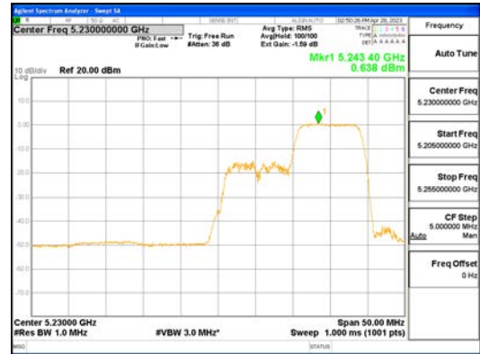
ANT1_802.11ax_HE40_106T_High_UNI I 1
