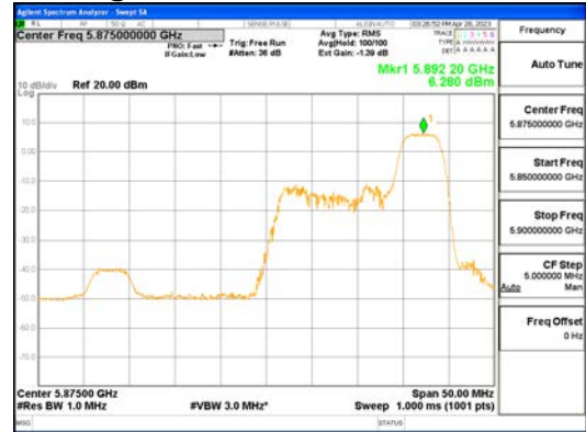
ANTO_802.11ax_HE40_52T_High_UNI 4
