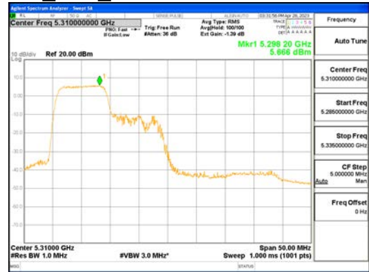
ANTO_802.11ax_HE40_106T_Low_UNII 2A
