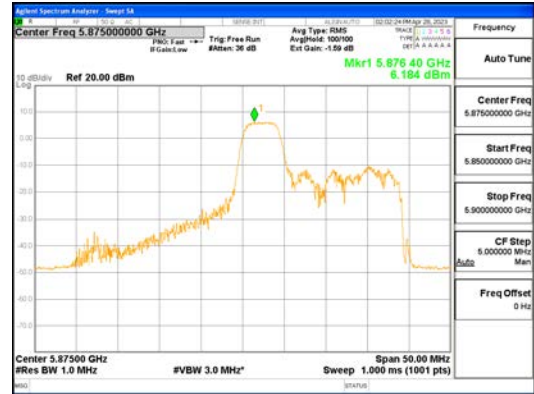
ANT1_802.11ax_HE40_52T_Mid_UNI I 4
