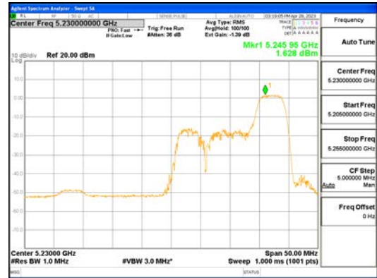
ANTO_802.11ax_HE40_52T_High_UNI 1
