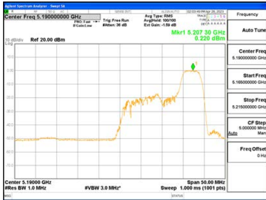
ANT1_802.11ax_HE40_52T_High_UNI 1
