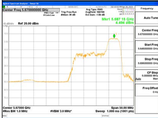
ANT1_802.11ax_HE40_52T_High_UNI 1C
