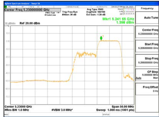
ANTO_802.11ax_HE40_106T_High_UNI I 1
