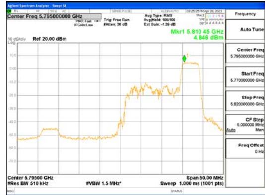
ANTO_802.11ax_HE40_52T_High_UNI 3
