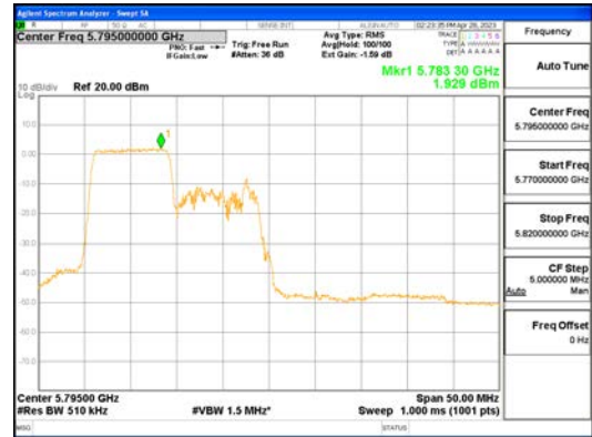
ANT1_802.11ax_HE40_106T_Low_UNI1 3
