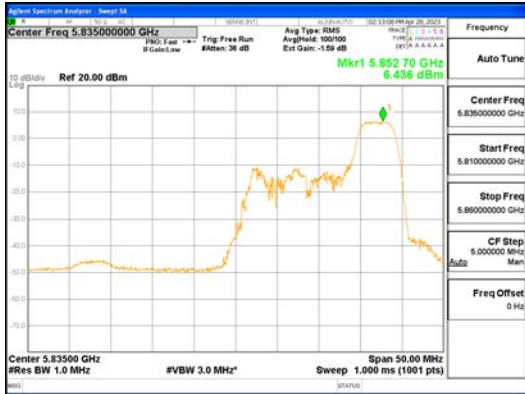
ANT1_802.11ax_HE40_52T_High_UNI 4
