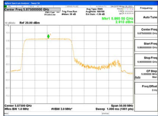
ANTO_802.11ax_HE40_242T_Low_UNI I 4
