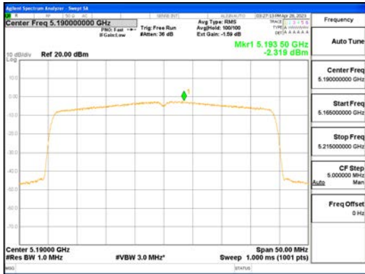
ANT1_802.11ax_HE40_484T_UNI I
