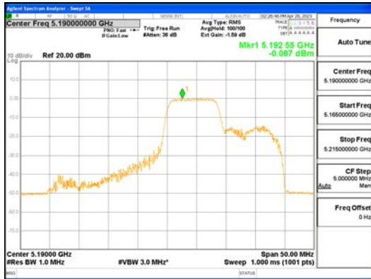
ANT1_802.11ax_HE40_106T_Mid_UNI 1
