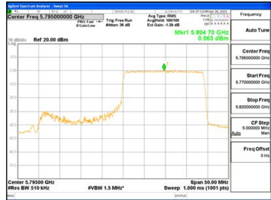
ANTO_802.11ax_HE40_242T_High_UNI I 3
