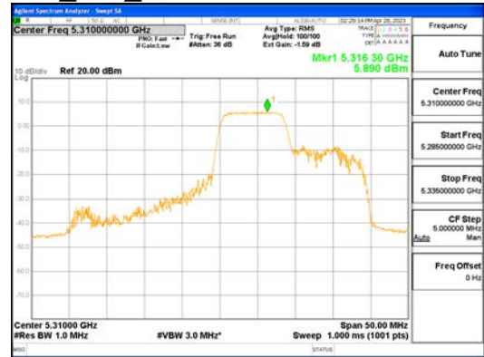
ANT1_802.11ax_HE40_106T_Mid_UNI 2A
