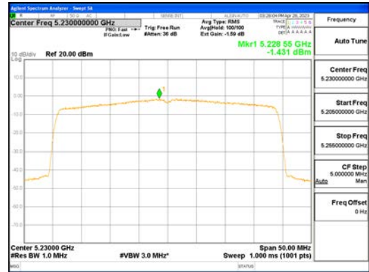
ANT1_802.11ax_HE40_484T_UNI I
