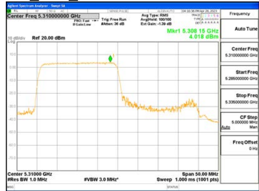
ANTO_802.11ax_HE40_242T_Low_UNII 2A
