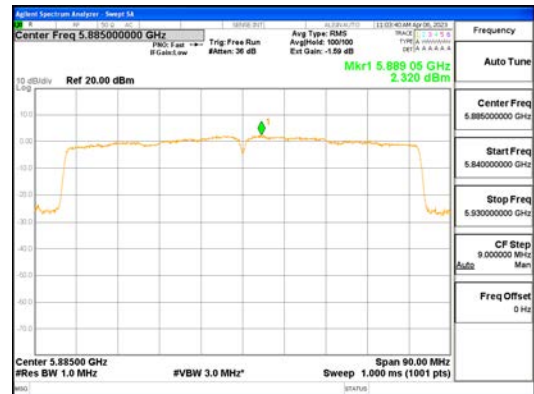
ANT1_802.11ac_VHT80_UNII 4
