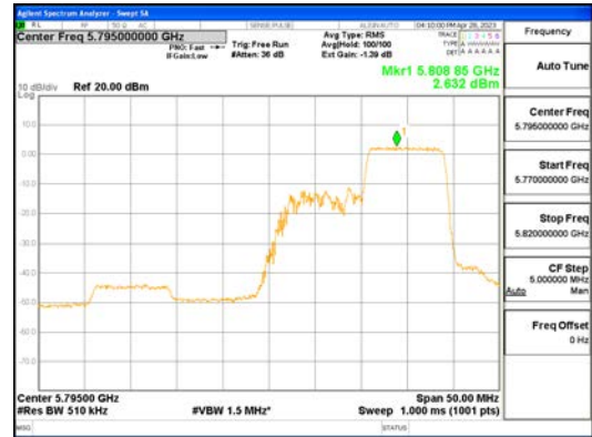
ANTO_802.11ax_HE40_106T_High_UNI I 3
