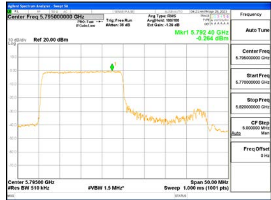
ANTO_802.11ax_HE40_242T_Low_UNI I 3
