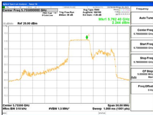
ANTO_802.11ax_HE40_106T_Mid_UNI I 3
