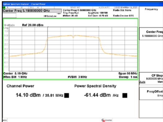
ANT2_802.11ac_VHT40_UNI1
