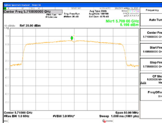
ANT2_802.11ax_HE40_SU_UNI1 2C
