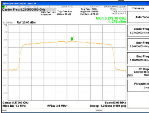
ANT1_802.11ax_HE40_SU_UNI1 2A
