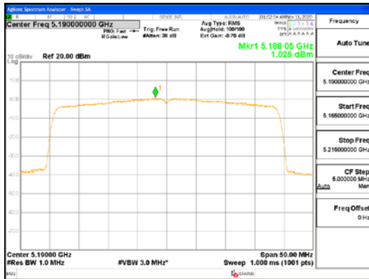
ANT2_802.11ax_HE40_SU_UNI1 1
