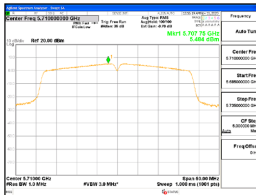
ANT2_802.11n_HT40_UNII 2C
