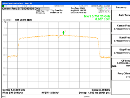
ANT1_802.11ax_HE40_SU_UNI I 3
