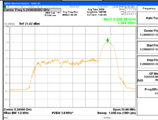
ANT1_802.11ax_HE20_26T_High_UNI 1
