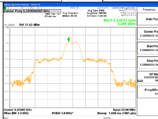
ANT1_802.11ax_HE20_26T_Mid_UNI1 2A
