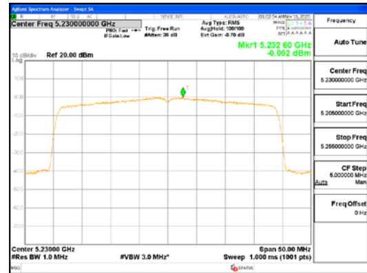
ANT2_802.11ax_HE40_SU_UNI1 1
