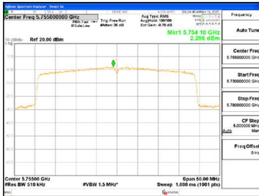
ANT2_802.11ax_HE40_SU_UNI I 3
