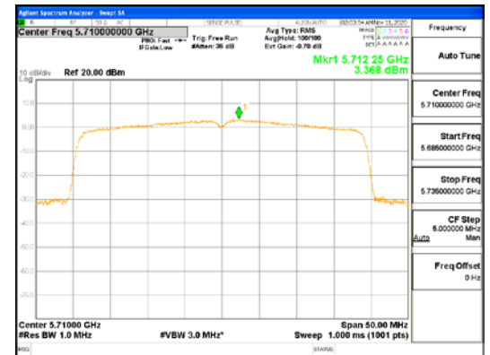
ANT1_802.11ax_HE40_SU_UNI1 2C
