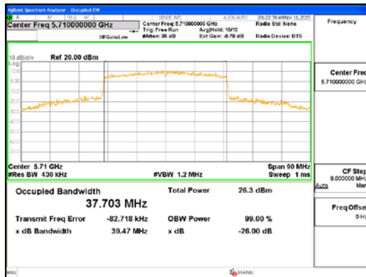
ANT2_802.11ax_HE40_SU_UNI1 2C
