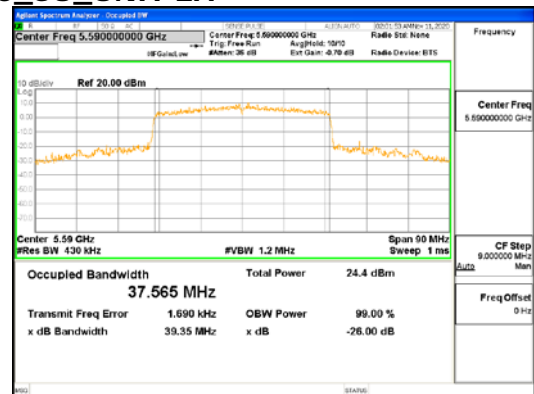
ANT1_802.11ax_HE40_SU_UNI1 2C
