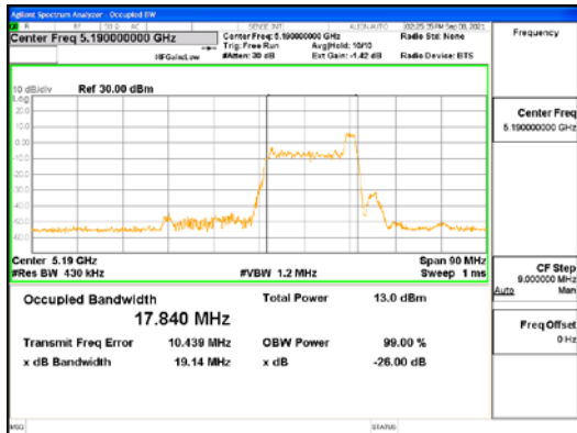
ANT1_802.11ax_HE40_26T_High_UNI 1
