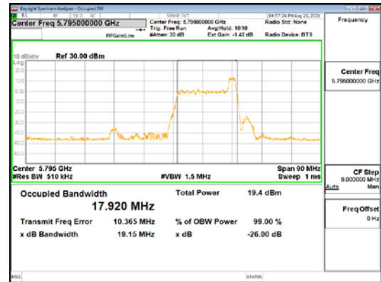
ANT2_802.11ax_HE40_26T_High_UNI I 3
