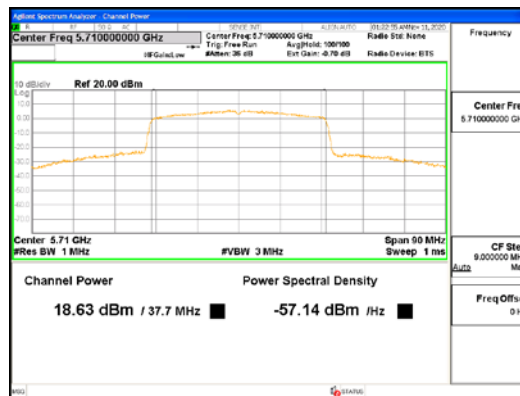
ANT2_802.11ax_HE40_UNI 2C
