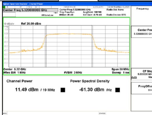
ANT1_802.11ax_HE20_UNI1 2A
