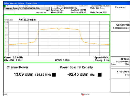
ANT2_802.11ac_VHT40_UNI1 1
