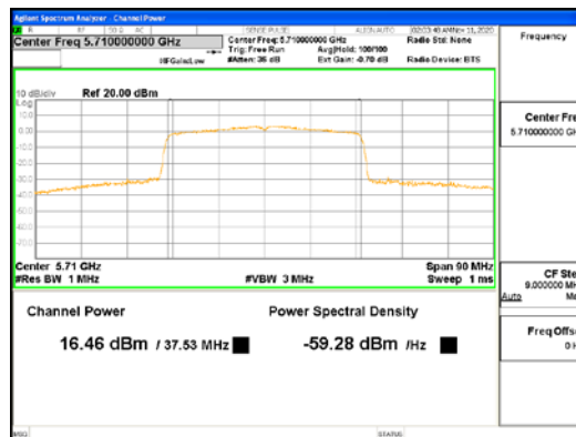
ANT1_802.11ax_HE40_UNI 2C
