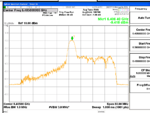
ANT1_802.11ax_HE40_26T_Mid_UNII 5
