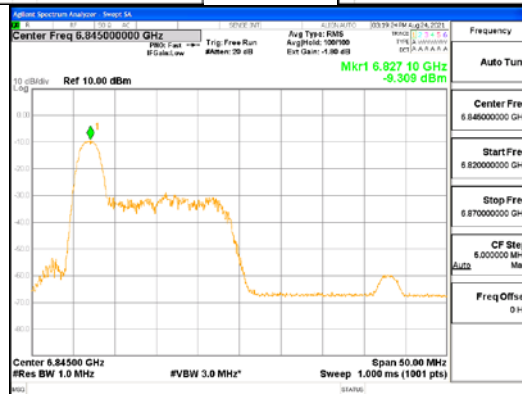
ANT1_802.11ax_HE40_26T_Low_UNII 7
