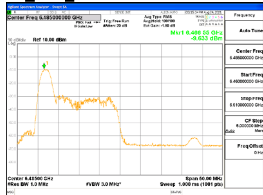
ANT1_802.11ax_HE40_26T_Low_UNII 6
