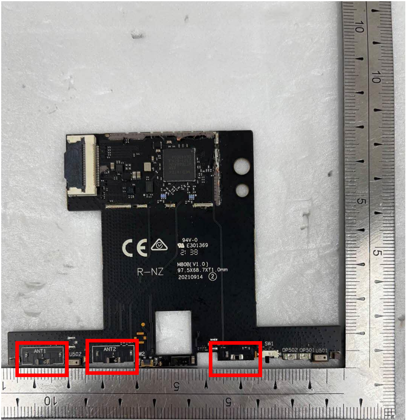
Chip Antenna
