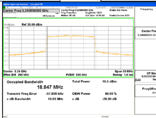
ANT1_802.11ax_HE20_SU_UNI 1
