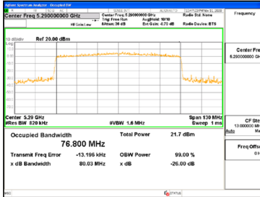
ANT2_802.11ax_HE80_SU_UNII 2A
