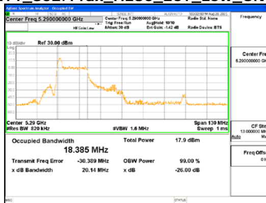
ANT1_802.11ax_HE80_26T_Low_UNII 2A
