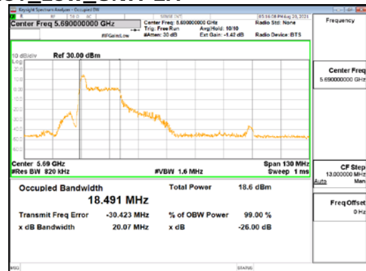
ANT2_802.11ax_HE80_26T_Low_UNII 2C
