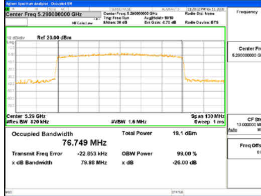
ANT1_802.11ax_HE80_SU_UNII 2A
