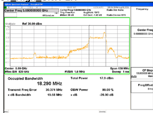
ANT1_802.11ax_HE80_26T_High_UNI 2C
