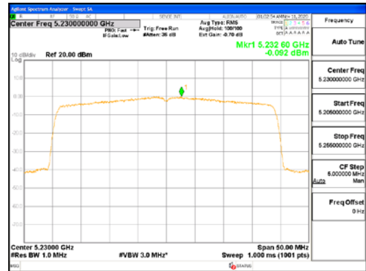
ANT2_802.11ax_HE40_SU_UNI1 1
