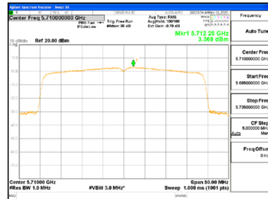
ANT1_802.11ax_HE40_SU_UNI1 2C
