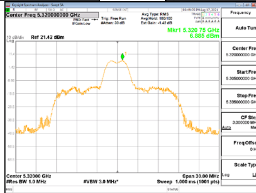
ANT2_802.11ax_HE20_26T_Mid_UNII 2A
