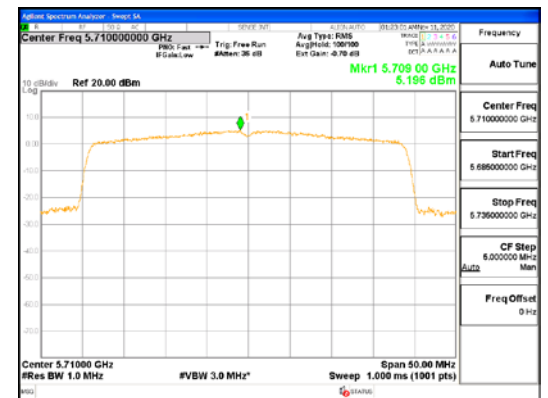
ANT2_802.11ax_HE40_SU_UNI1 2C
