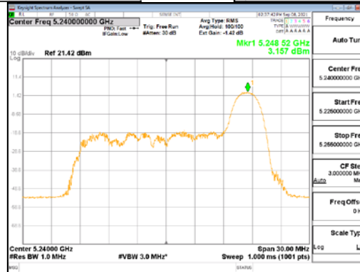
ANT2_802.11ax_HE20_26T_High_UNI 1
