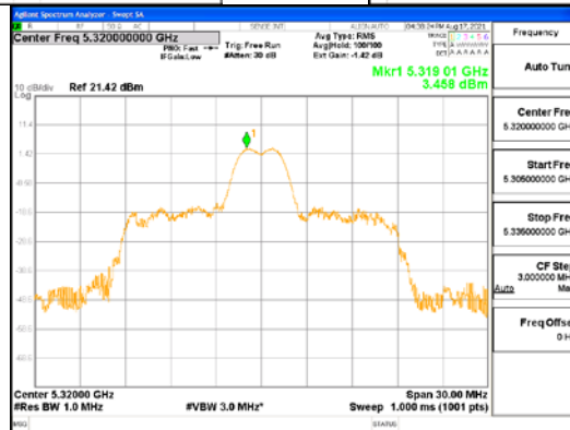
ANT1_802.11ax_HE20_26T_Mid_UNI1 2A
