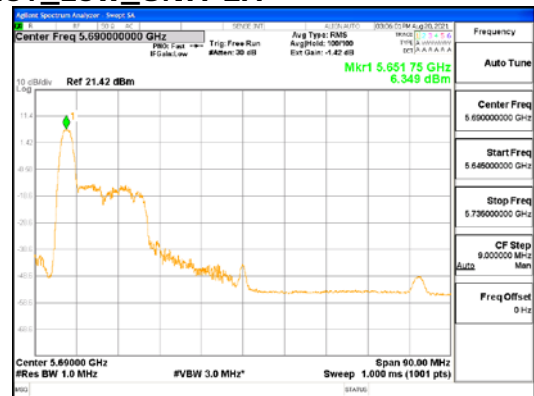
ANT1_802.11ax_HE80_26T_Low_UNII 2C
