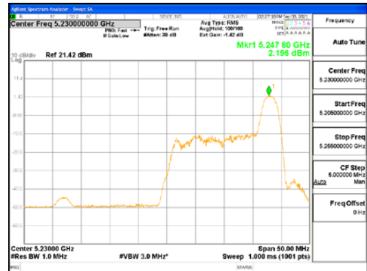
ANT1_802.11ax_HE40_26T_High_UNI 1
