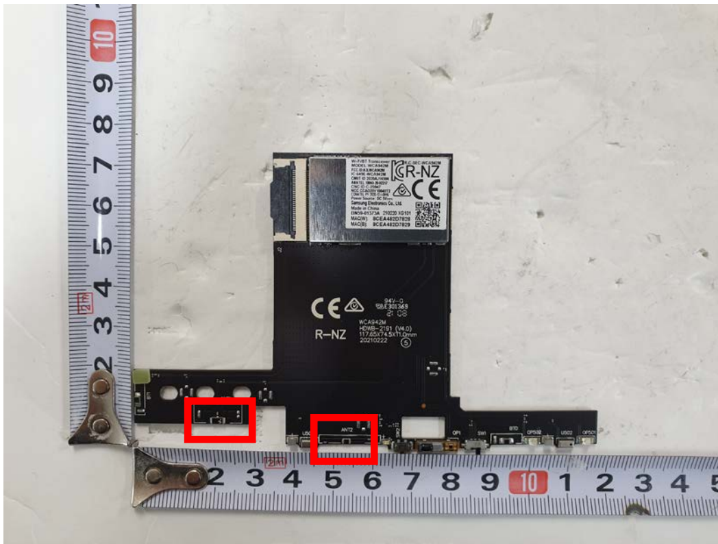
WLAN Antenna
