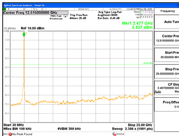
ANT2, 802.11ax_HE20
