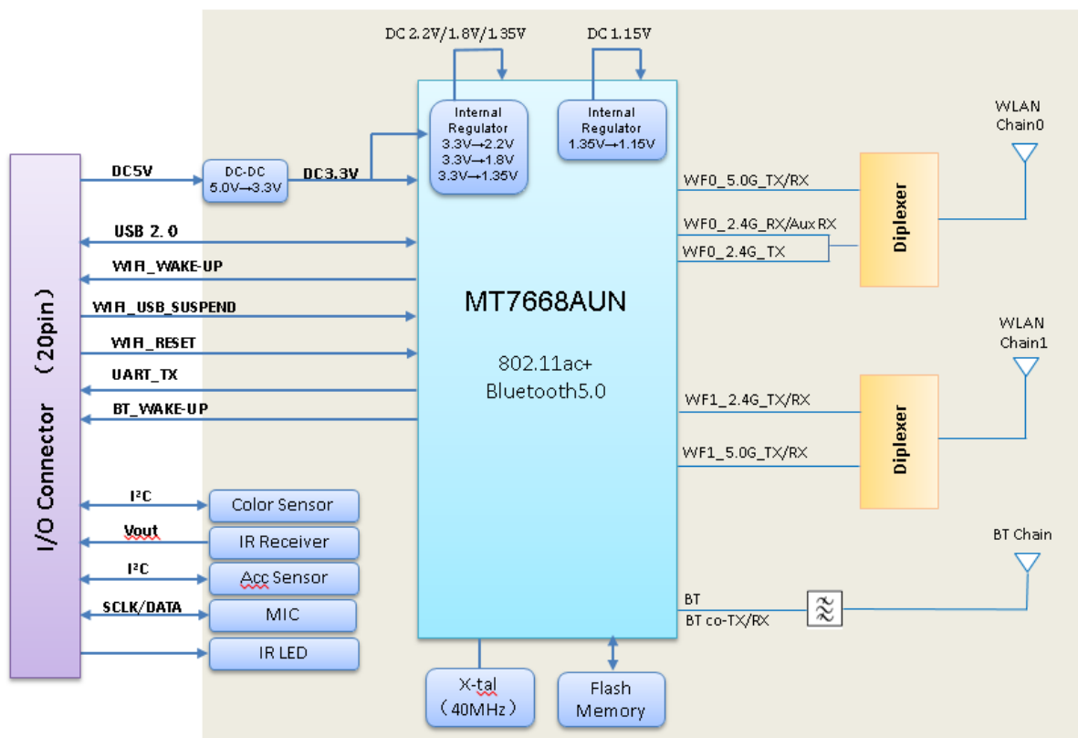
Figure 1-1 WCA732M block diagram and System Interface
