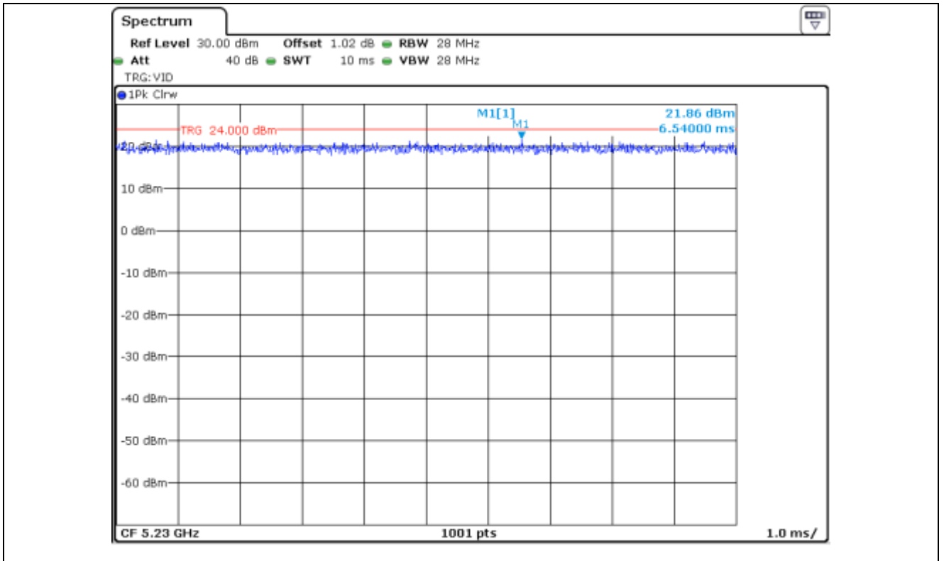
UNII 1_802.11 HT40_Antenna 1
