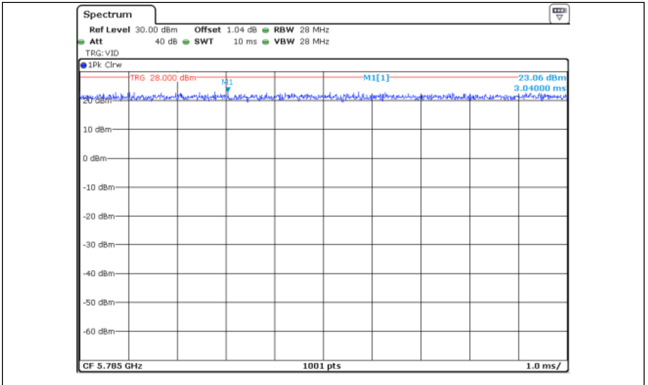
UNII 3_802.11 a_Antenna 0
