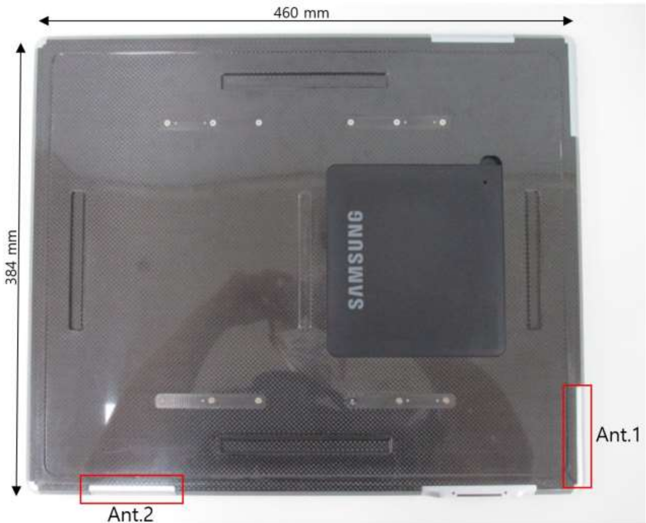
Figure E-1 Antenna Location (Rear Side View)
