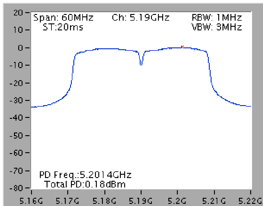
Power Density Plot on Configuration IEEE 802.11n MCS0 40MHz / Ant. 1 &amp; Ant. 2 / 5190 MHz
