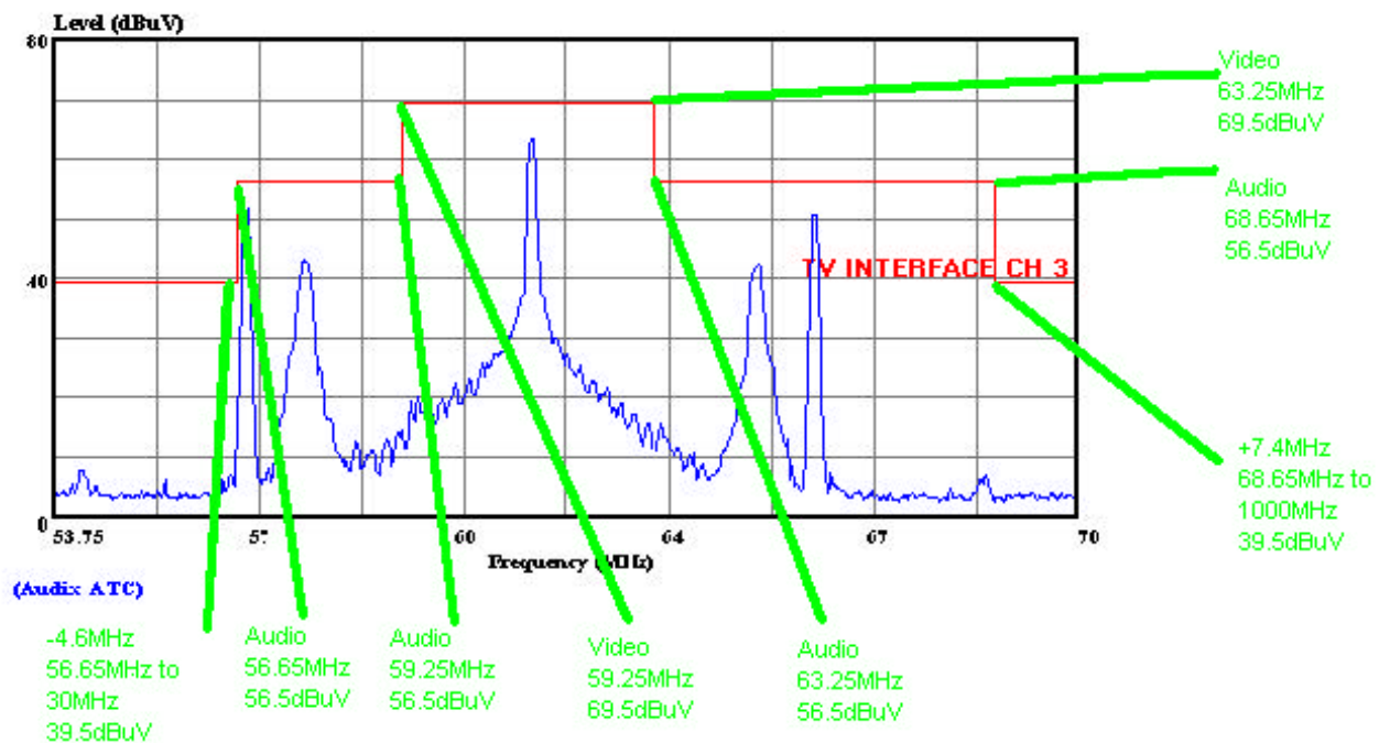
CHANNEL 3 EMISSION MASK FCC 15.115(b)(1)(ii) & 15.115(b)(2)(ii).
