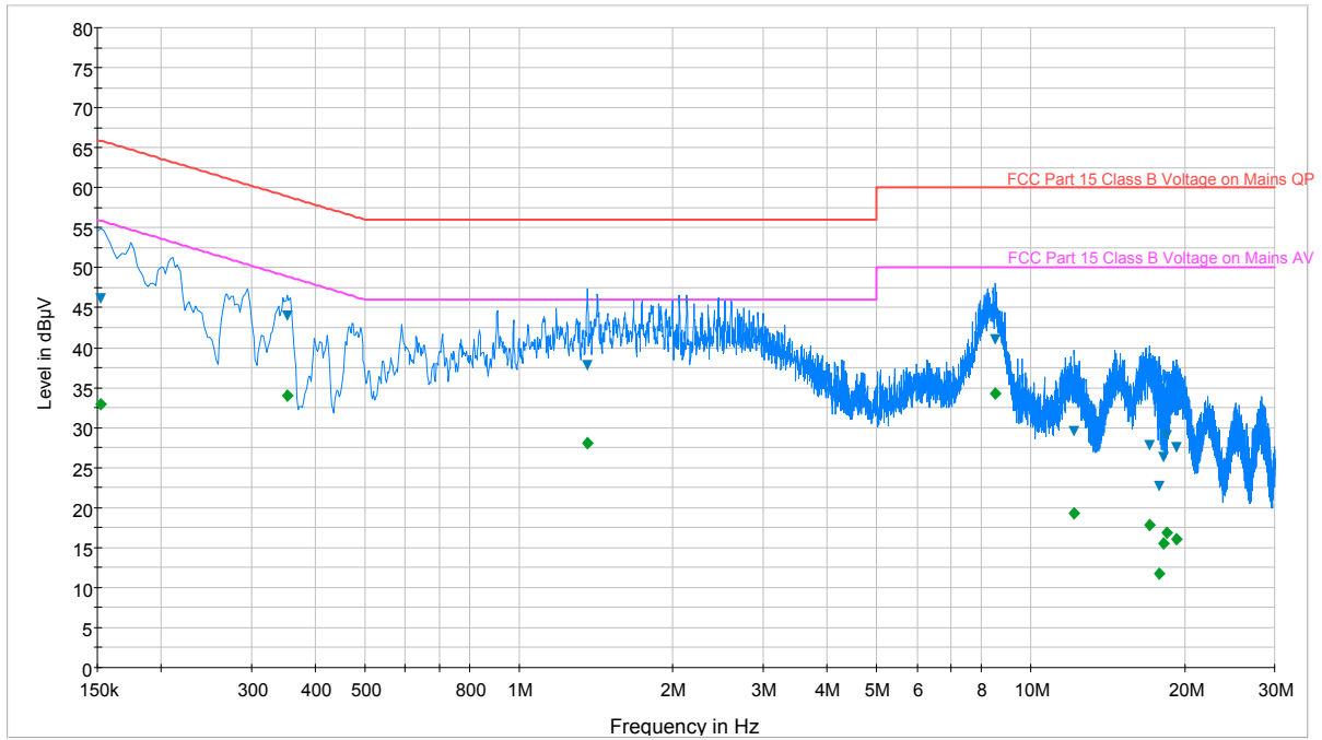
Plot 6-15. Line Conducted Plot with Bluetooth LE (L1)
