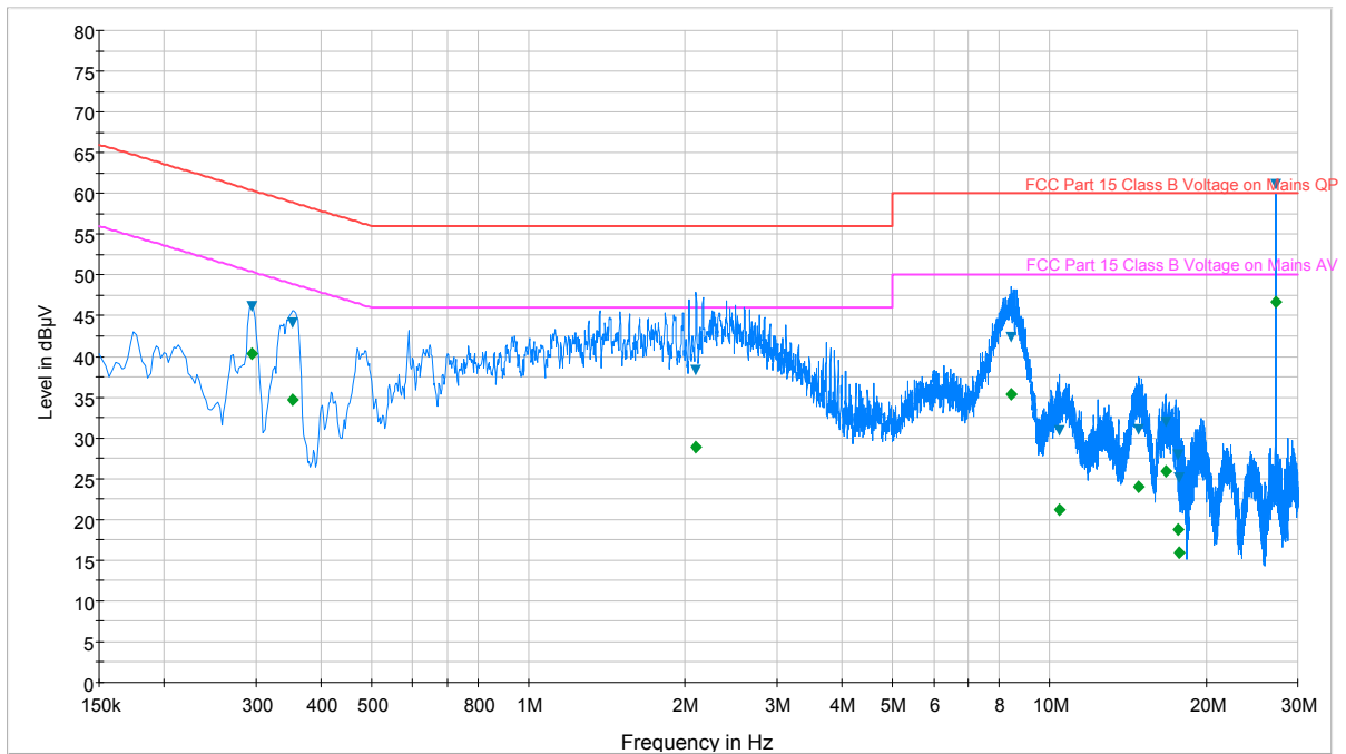
Plot 6-59. Line Conducted Plot with 802.11b (L1)
