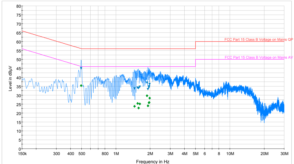
Plot 6-25. Line-Conducted Test Plot (N)
