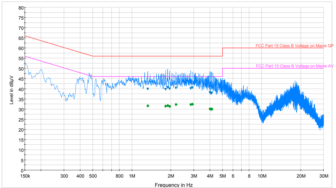
Plot 6-24. Line-Conducted Test Plot (L1)
