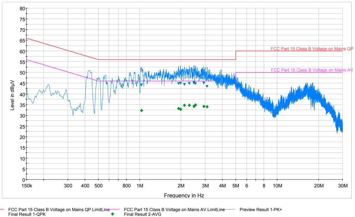
Plot 6-16. Line Conducted Plot with Bluetooth (LE, LN)
