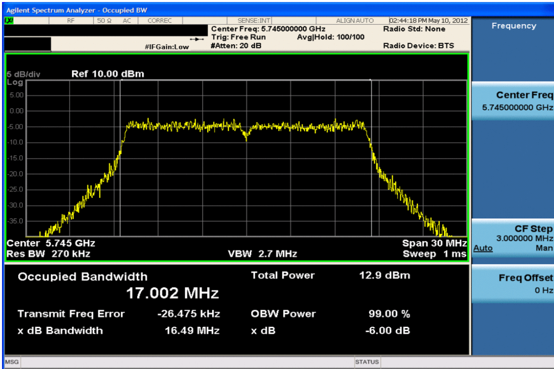
Plot 6-10. 6dB Bandwidth Plot (802.11a – Ch. 149)
