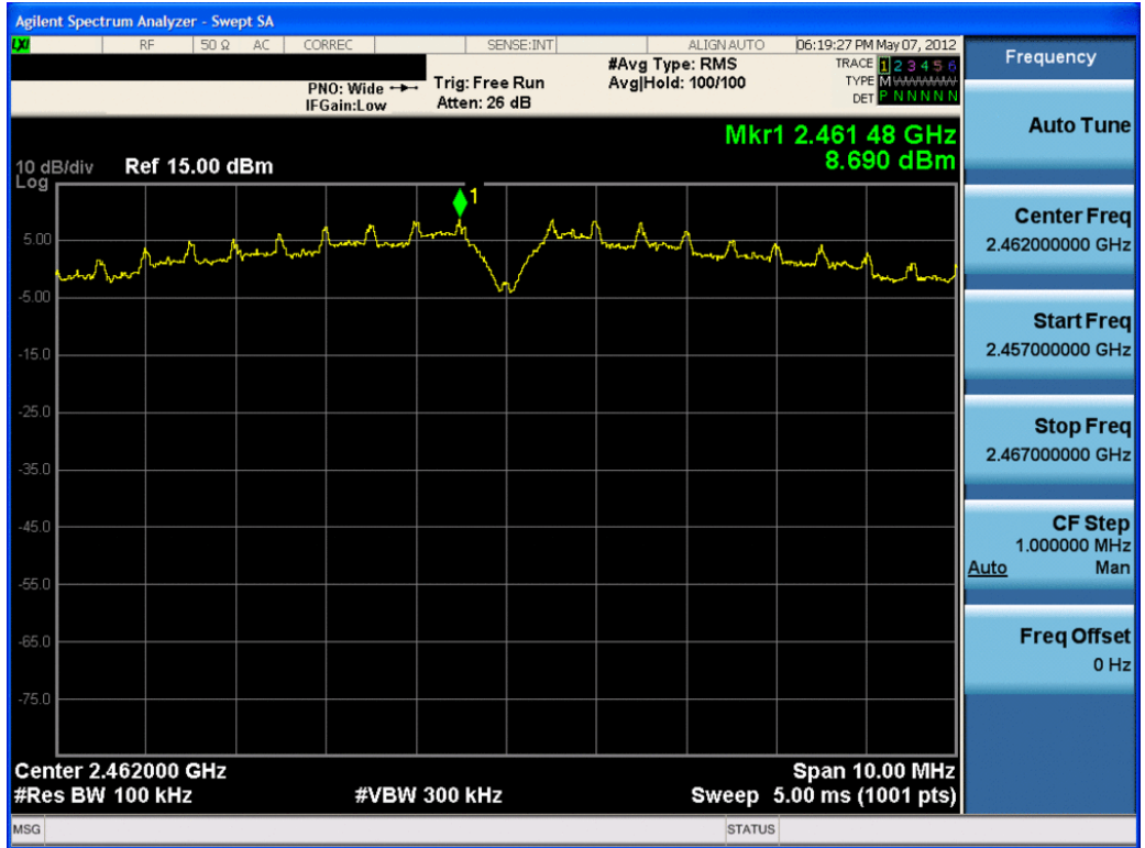
Plot 6-20. Power Spectral Density Plot (802.11b – Ch. 11)
