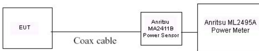
Figure 6-3. Test Instrument & Measurement Setup
