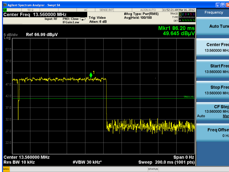
Plot 8-5. Line-Conducted Test Plot –Average Measurement at Fundamental - Line A
