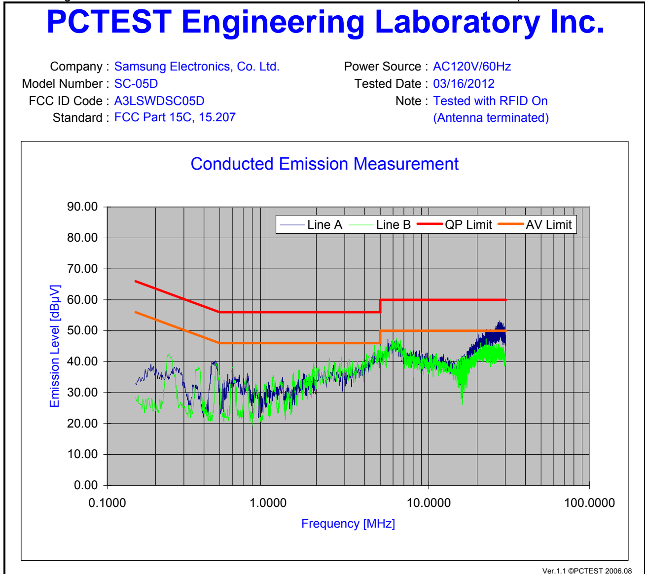
Plot 8-1. Line-Conducted Test Plot
