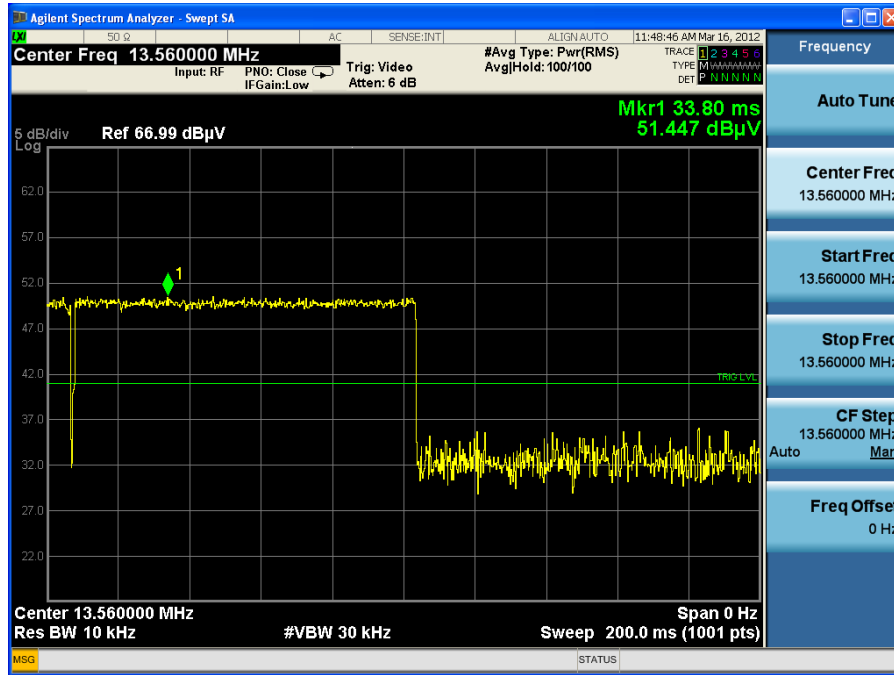
Plot 8-4. Line-Conducted Test Plot –Peak Measurement at Fundamental - Line A
