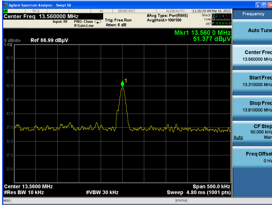
Plot 8-2. Line-Conducted Test Plot – RFID at 13.56MHz Line A
