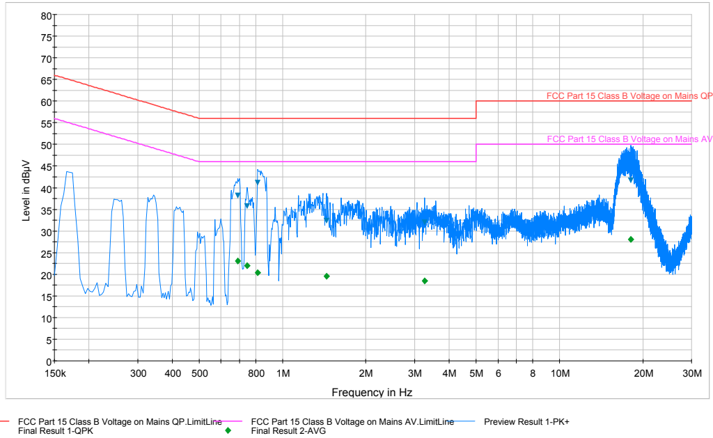
Plot 6-137. Line Conducted Plot with 802.11b (L1)
