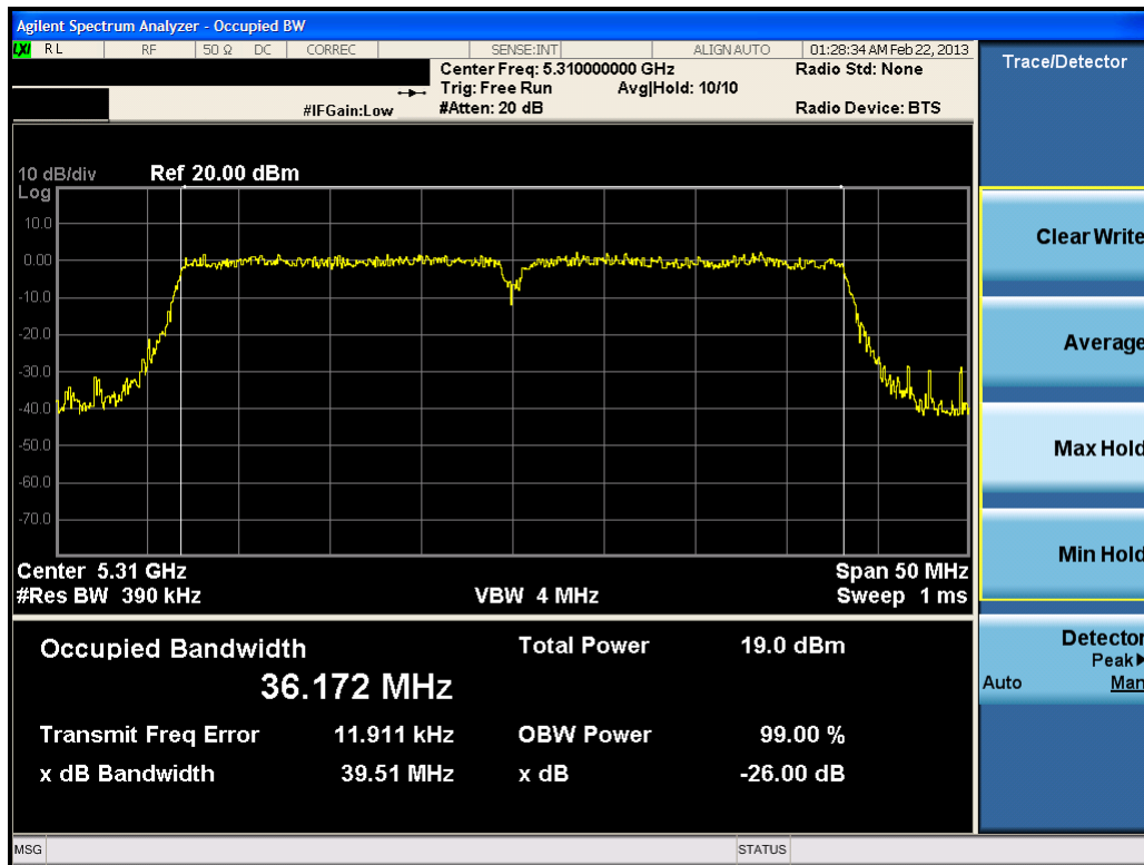
Plot 6-18. 26dB Bandwidth Plot (40MHz BW 802.11n (UNII Band 2) – Ch. 62)
