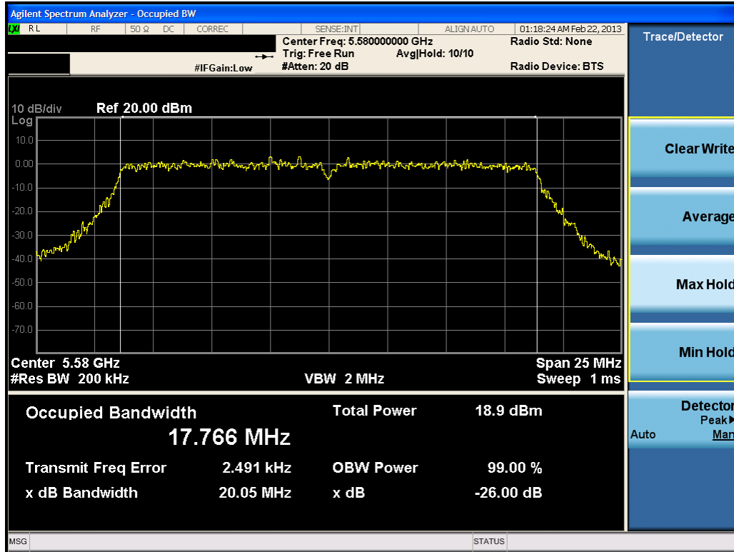
Plot 6-25. 26dB Bandwidth Plot (20MHz BW 802.11n (UNII Band 3) – Ch. 116)
