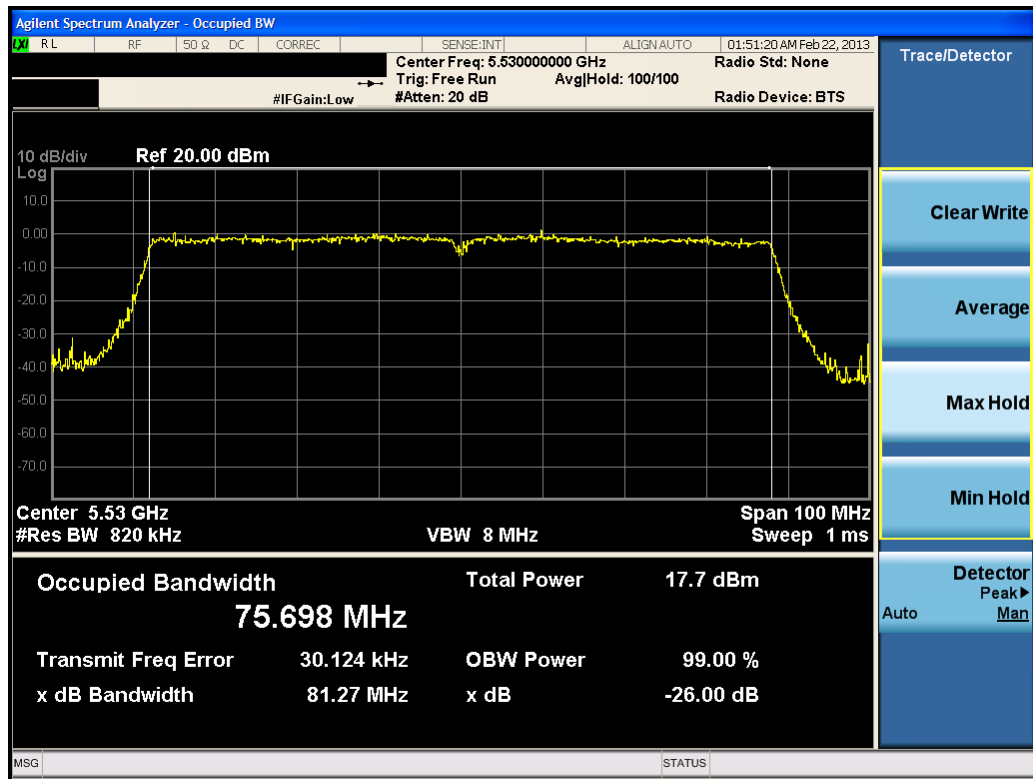
Plot 6-30. 26dB Bandwidth Plot (80MHz BW 802.11ac (UNII Band 3) – Ch. 106)
