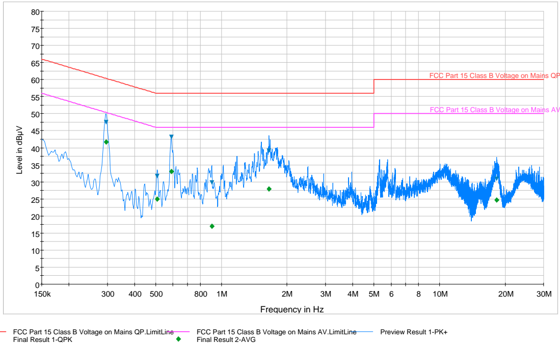
Plot 6-88. Line Conducted Plot with 802.11a UNII Band 3 (L1)
