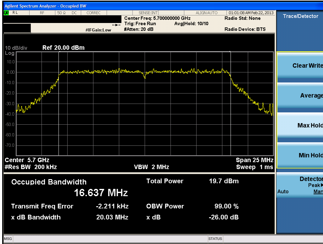
Plot 6-23. 26dB Bandwidth Plot (802.11a (UNII Band 3) – Ch. 140)
