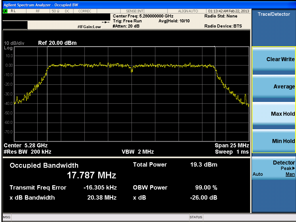
Plot 6-15. 26dB Bandwidth Plot (20MHz BW 802.11n (UNII Band 2) – Ch. 56)
