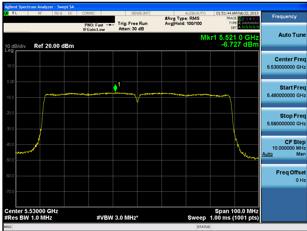
Plot 6-59. Peak Power Spectral Density Plot (80MHz BW 802.11ac (UNII Band 3) – Ch. 106)
