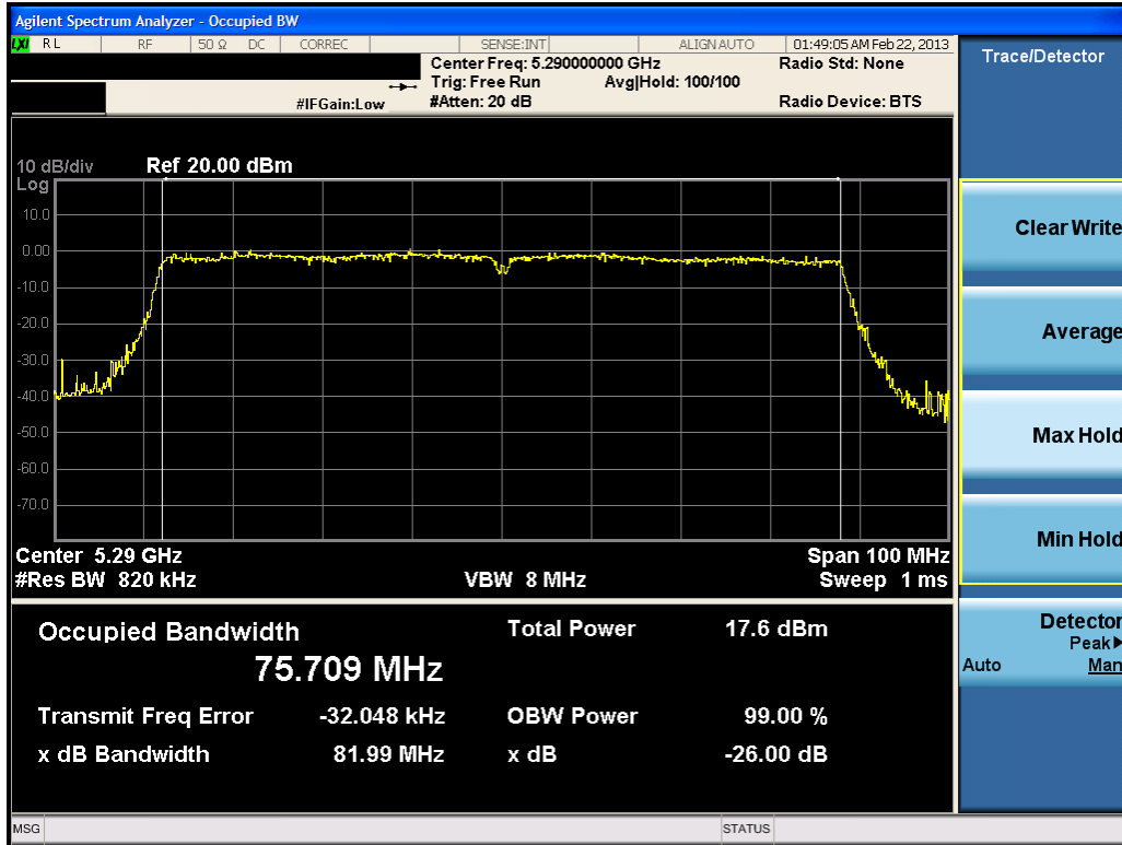
Plot 6-19. 26dB Bandwidth Plot (80MHz BW 802.11ac (UNII Band 2) – Ch. 58)
