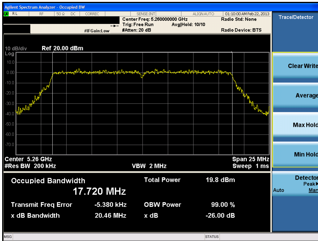
Plot 6-14. 26dB Bandwidth Plot (20MHz BW 802.11n (UNII Band 2) – Ch. 52)
