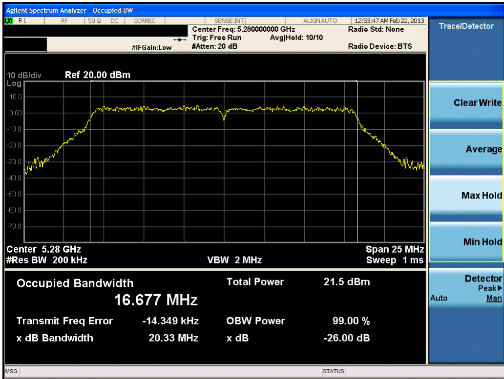
Plot 6-12. 26dB Bandwidth Plot (802.11a (UNII Band 2) – Ch. 56)
