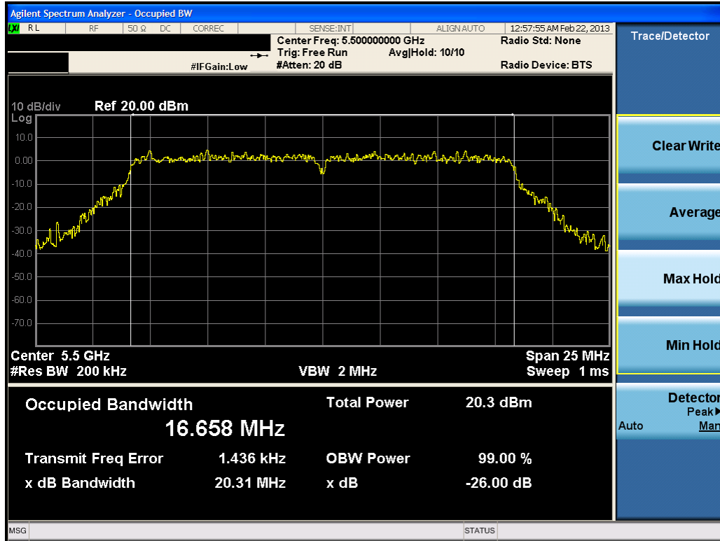
Plot 6-21. 26dB Bandwidth Plot (802.11a (UNII Band 3) – Ch. 100)
