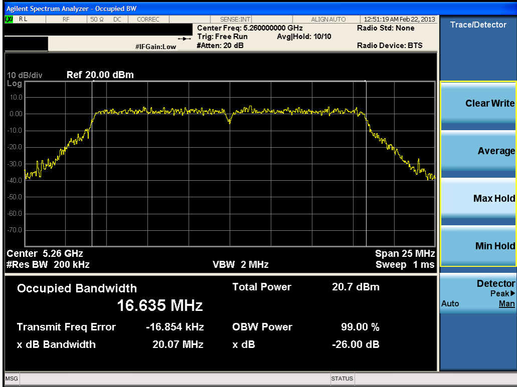
Plot 6-11. 26dB Bandwidth Plot (802.11a (UNII Band 2) – Ch. 52)
