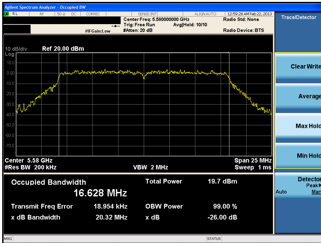
Plot 6-22. 26dB Bandwidth Plot (802.11a (UNII Band 3) – Ch. 116)
