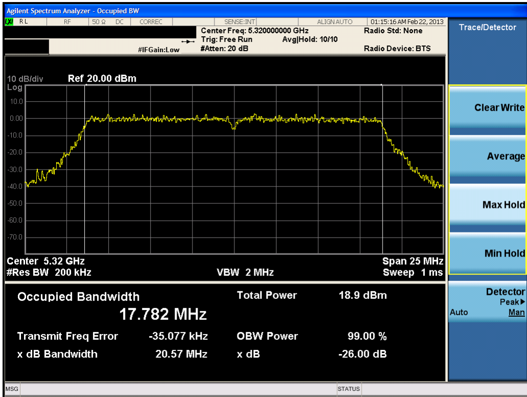
Plot 6-16. 26dB Bandwidth Plot (20MHz BW 802.11n (UNII Band 2) – Ch. 64)
