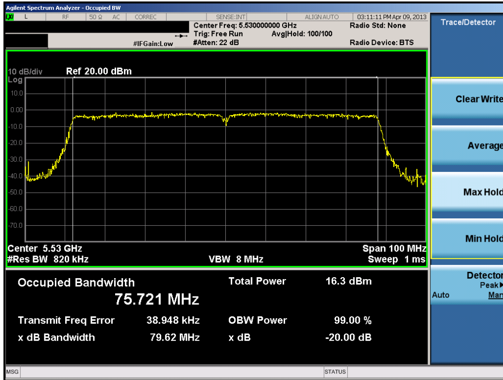
Plot 6-31. 20dB Bandwidth Plot (80MHz BW 802.11ac (UNII Band 3) – Ch. 106)
