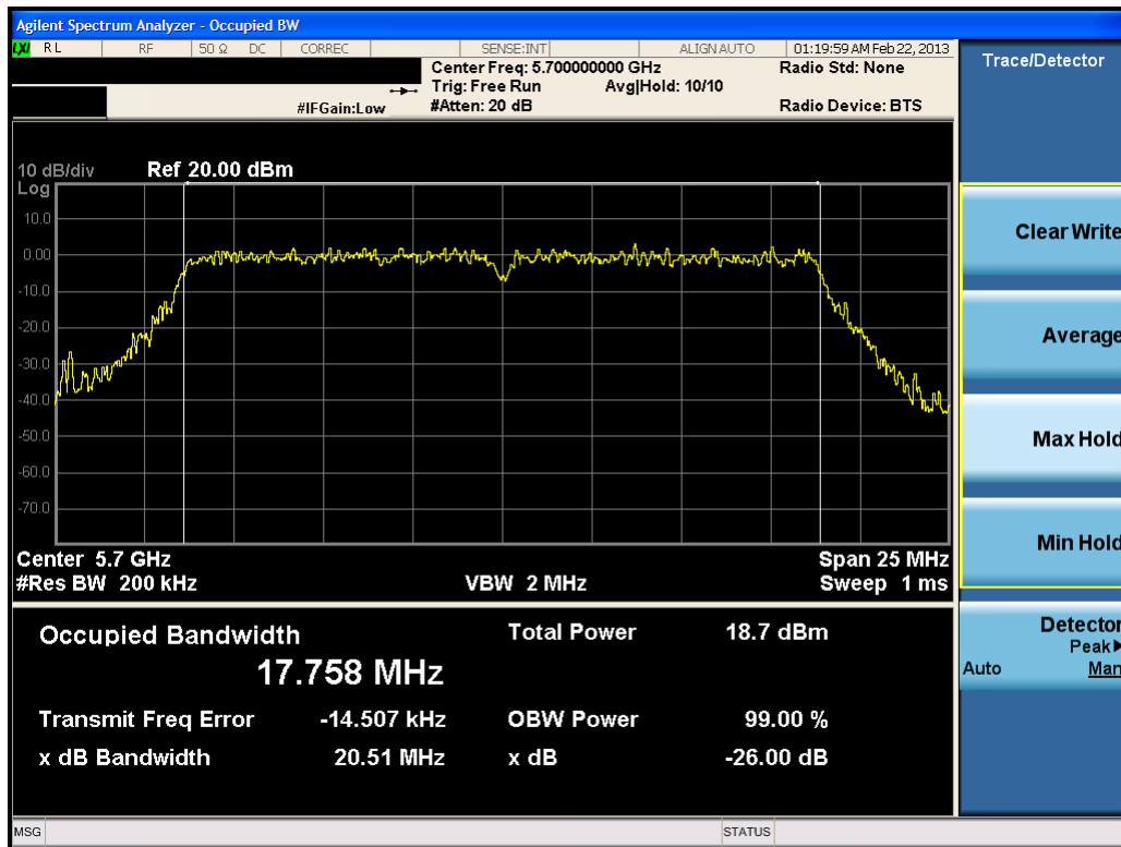
Plot 6-26. 26dB Bandwidth Plot (20MHz BW 802.11n (UNII Band 3) – Ch. 140)
