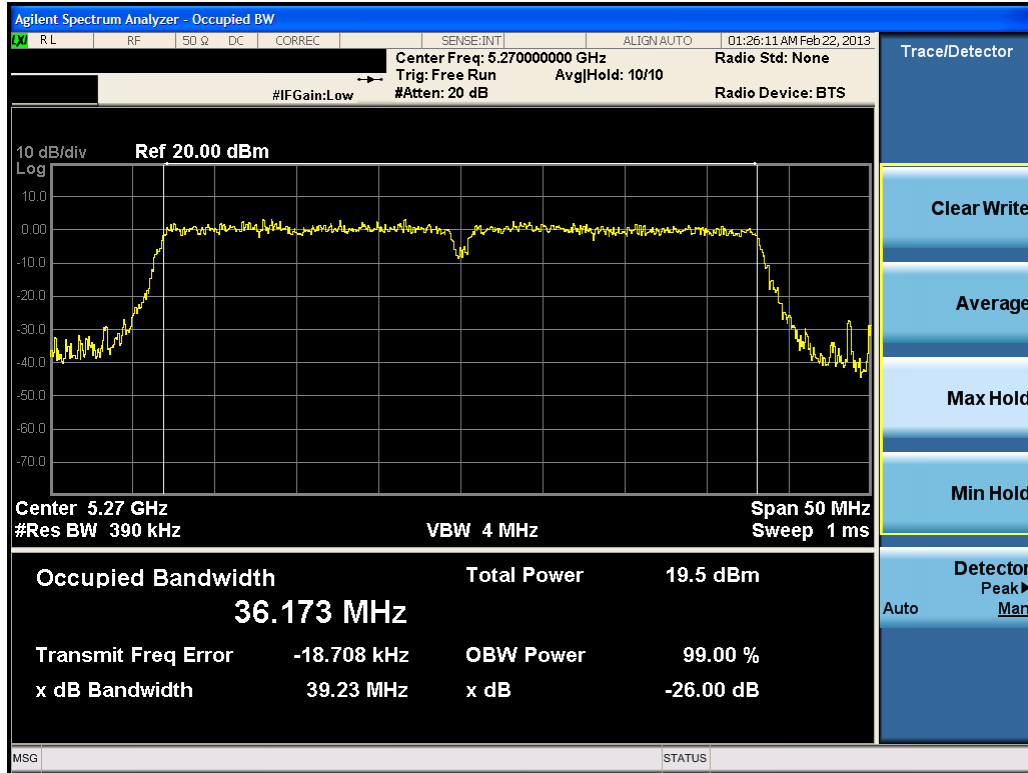
Plot 6-17. 26dB Bandwidth Plot (40MHz BW 802.11n (UNII Band 2) – Ch. 54)
