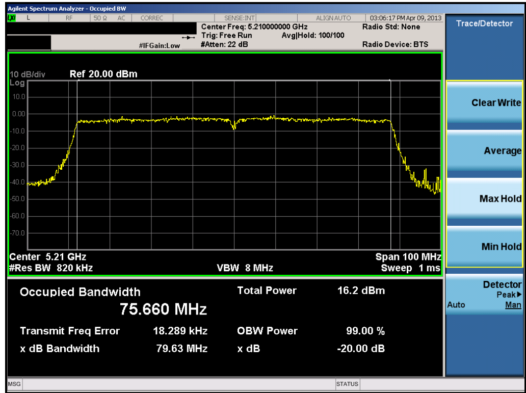
Plot 6-10. 20dB Bandwidth Plot (80MHz BW 802.11ac (UNII Band 1) – Ch. 42)
