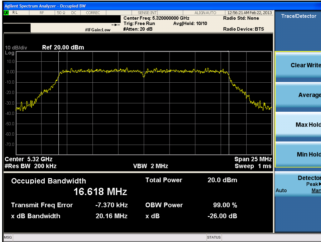
Plot 6-13. 26dB Bandwidth Plot (802.11a (UNII Band 2) – Ch. 64)
