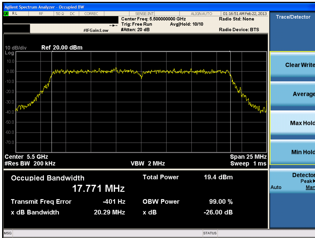
Plot 6-24. 26dB Bandwidth Plot (20MHz BW 802.11n (UNII Band 3) – Ch. 100)
