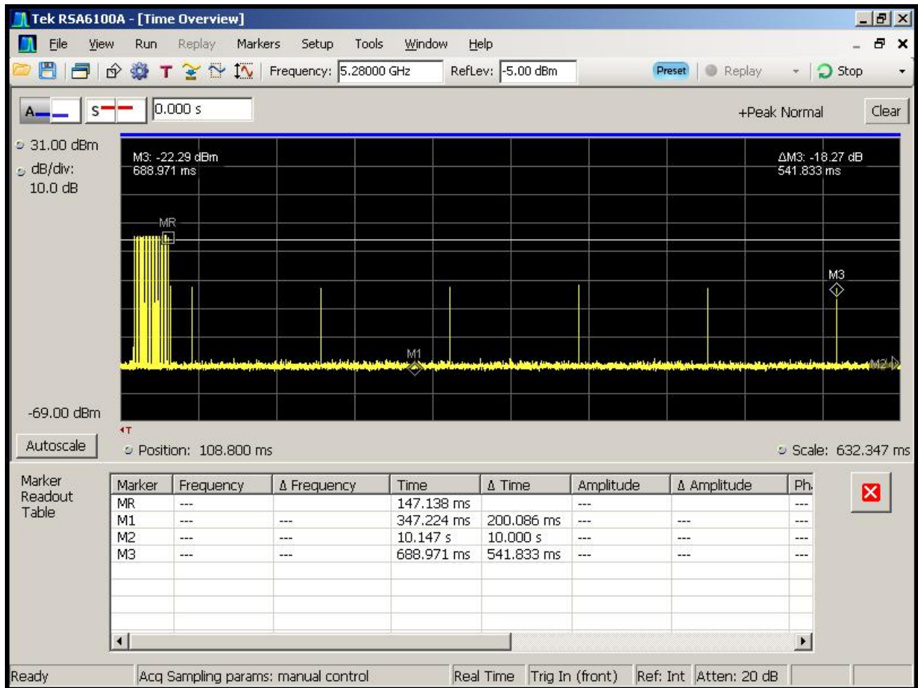
Figure 5-6. Aggregate Time
