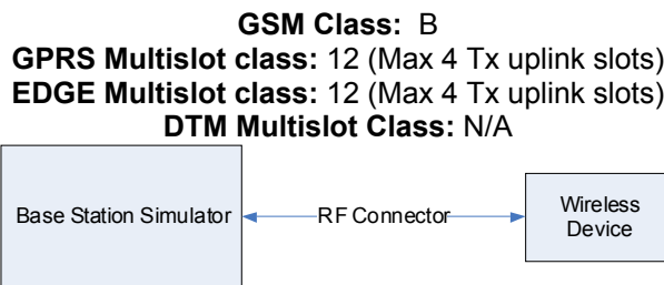
Figure 8-1 Power Measurement Setup
