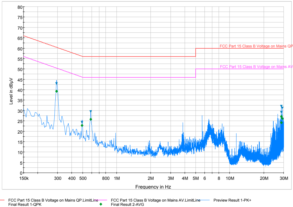
Plot 6-70. Line Conducted Plot with 802.11a (N)
