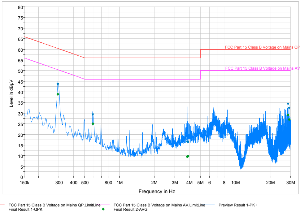
Plot 6-69. Line Conducted Plot with 802.11a (L1)
