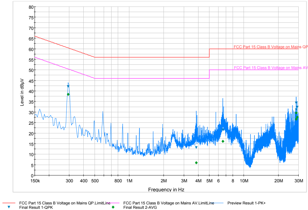
Plot 6-67. Line Conducted Plot with 802.11b (L1)
