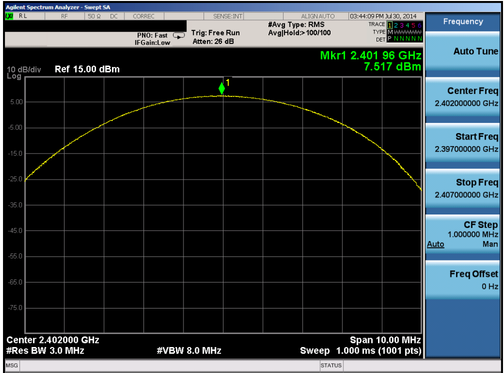
Plot 6-16. Peak Conducted Power (3Mbps – Ch. 0)
