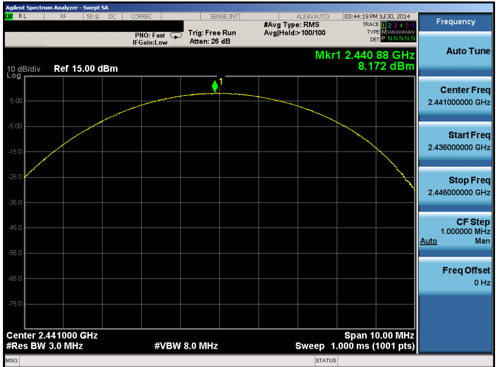
Plot 6-17. Peak Conducted Power (3Mbps – Ch. 39)
