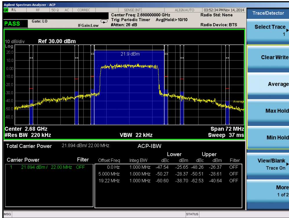
Plot 6-25. Upper ACP Plot (Band 41 – 20.0MHz QPSK – RB Size 100)
