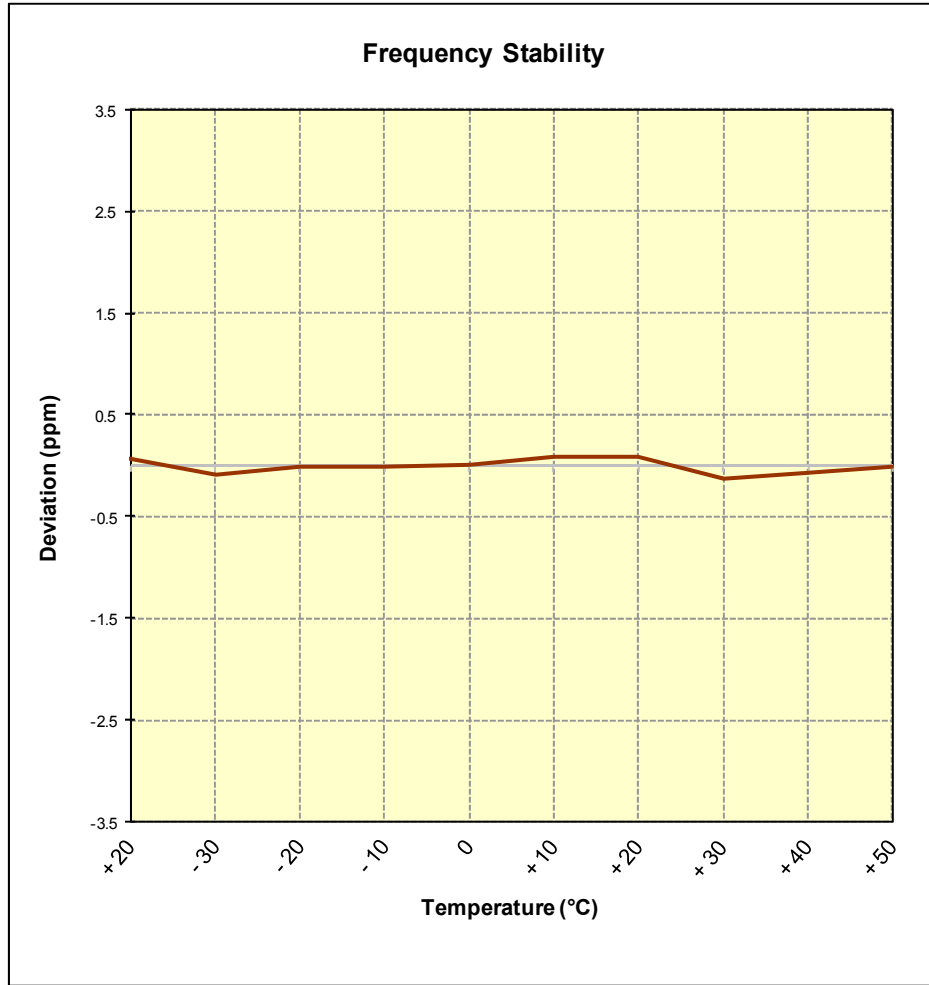
Figure 6-6. Frequency Stability Graph (Band 41)
