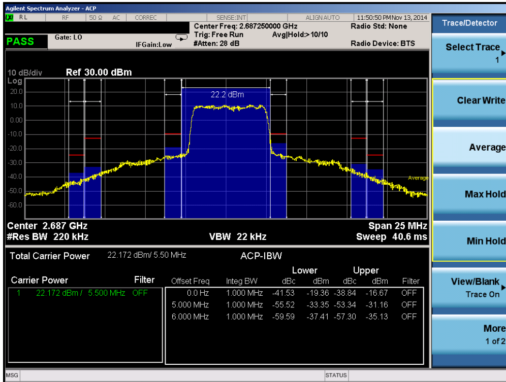
Plot 6-19. Upper ACP Plot (Band 41 – 5.0MHz QPSK – RB Size 25)
