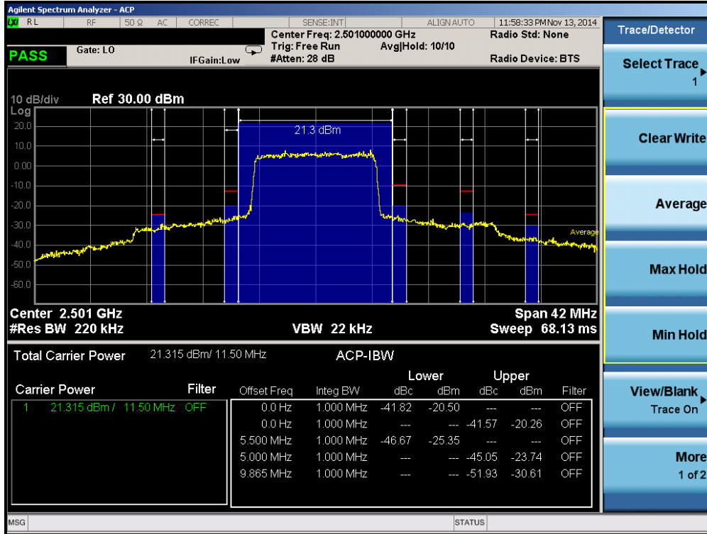
Plot 6-20. Lower ACP Plot (Band 41 – 10.0MHz QPSK – RB Size 50)
