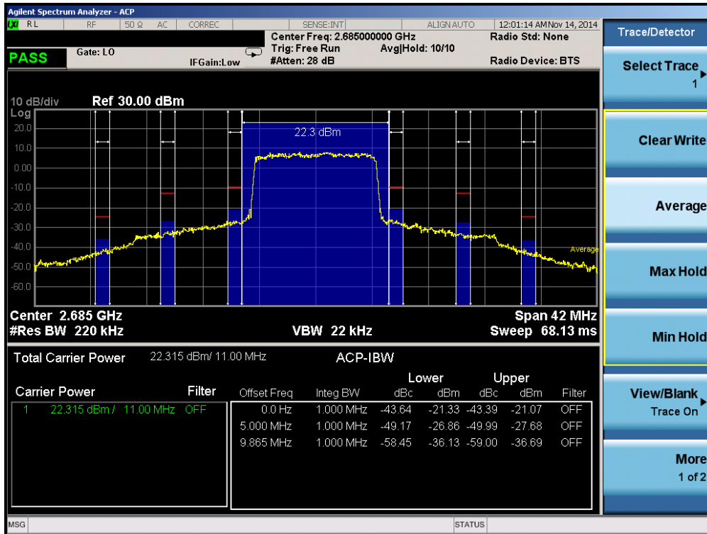
Plot 6-21. Upper ACP Plot (Band 41 – 10.0MHz QPSK – RB Size 50)
