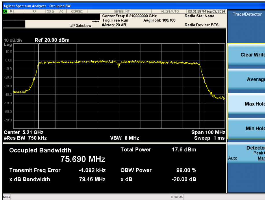
Plot 6-61. 20dB Bandwidth Plot (80MHz BW 802.11ac (UNII Band 1) – Ch. 42)
