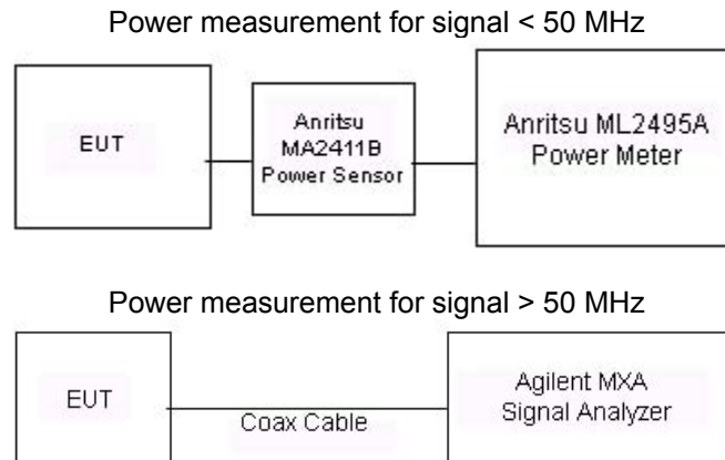
Figure 8-3 Power Measurement Setup
