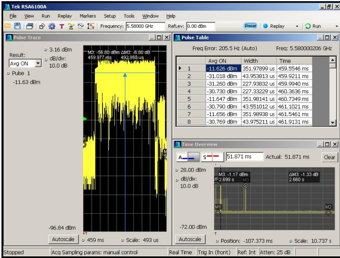
Figure 6-7. Pulse width analysis using Pulse Table and Pulse Trace Function
