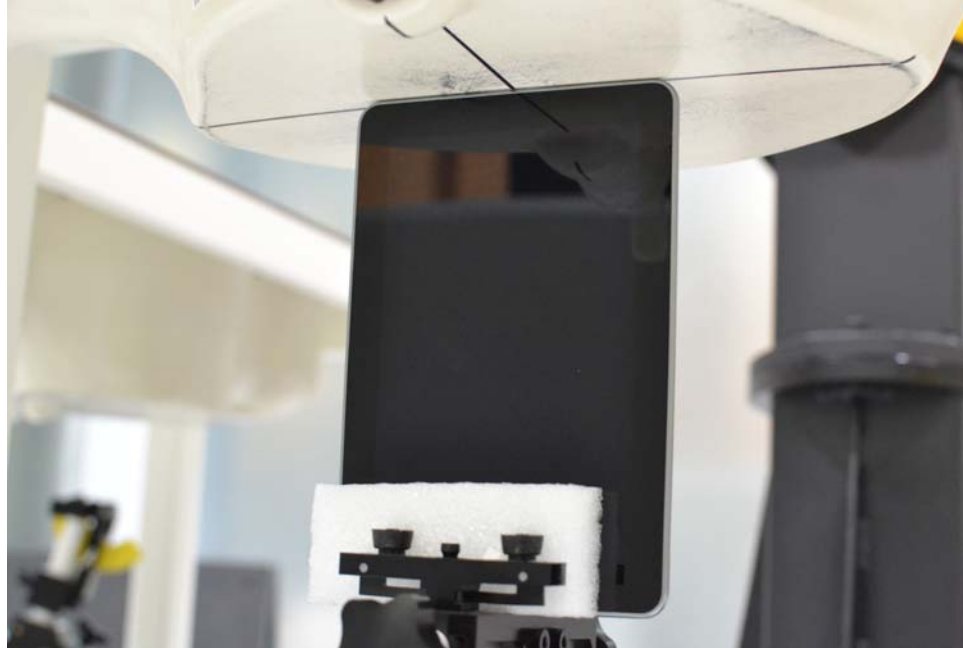
SAR Test Setup Photo 3: Bottom Edge at 0.0 cm
