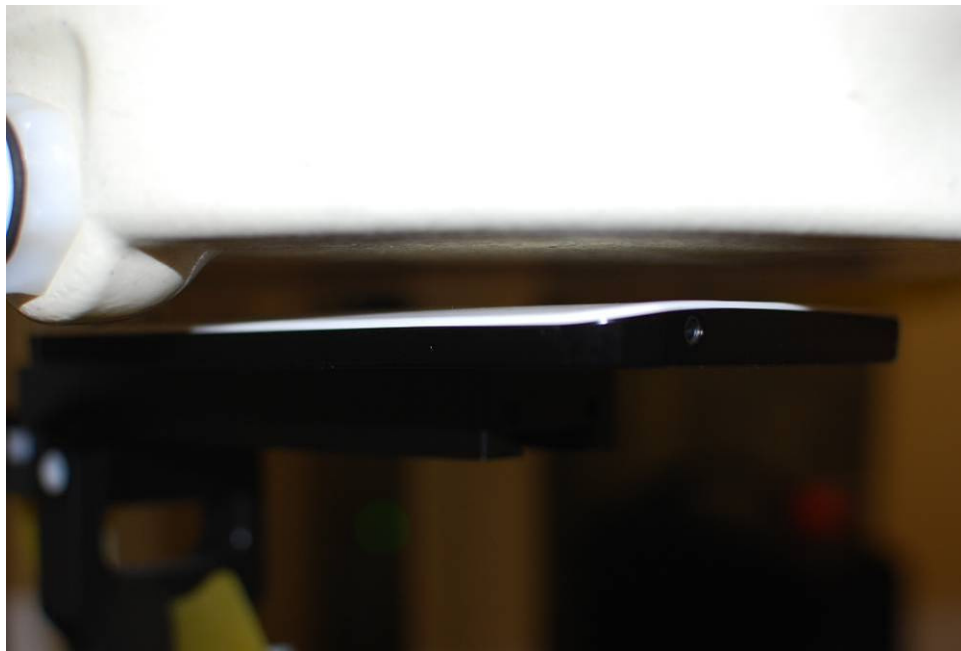
Figure 20-2 SAR Test Setup Photo 2 – Back Side at 1.0 cm (without power back-off)
