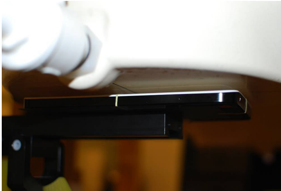
Figure 20-1 SAR Test Setup Photo 1 – Back Side at 0.5 cm (with power back-off)
