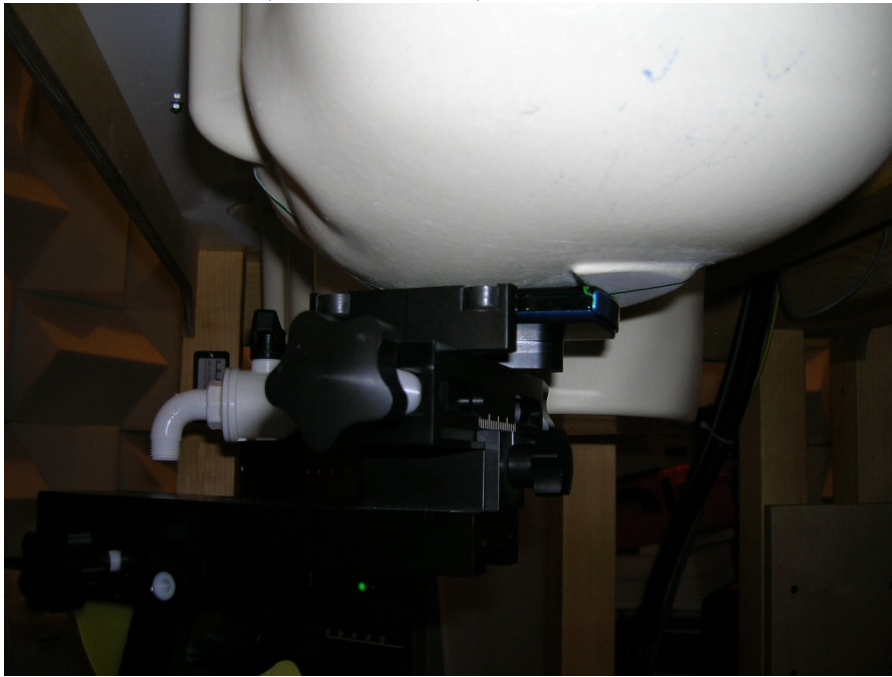
6. Left Head SAR, 15° Tilt, Slide In
