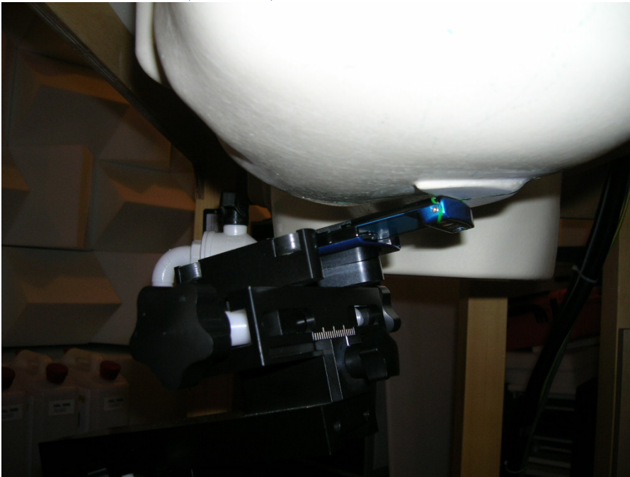
10. Left Head SAR, 15° Tilt, Slide Out
