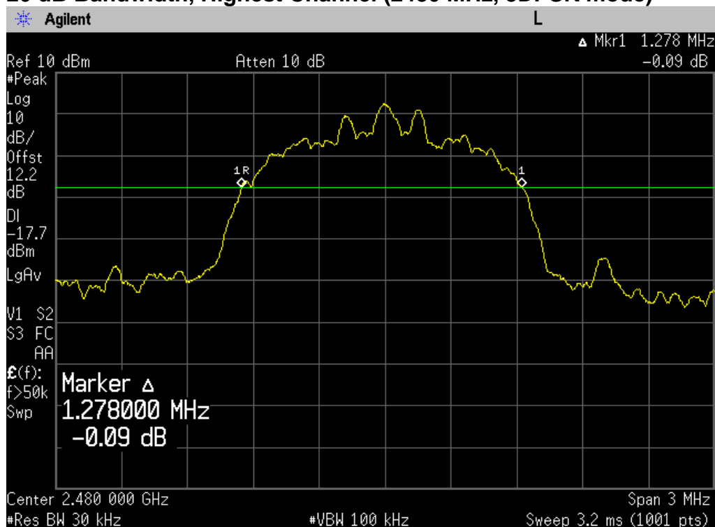
20 dB Bandwidth, Highest Channel (2480 MHz, 8DPSK mode)
