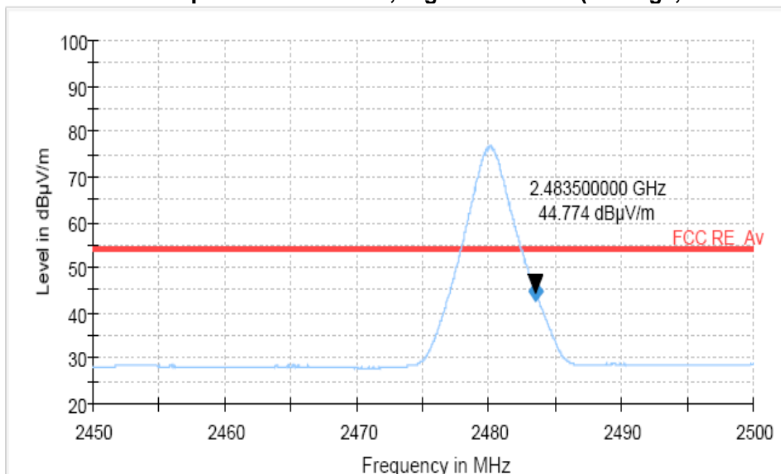
Restricted Band Spurious Emissions, Highest channel (Average, GFSK mode)
