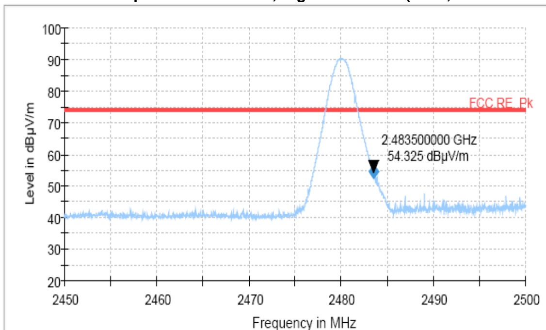
Restricted Band Spurious Emissions, Highest channel (Peak, 8DPSK mode)
