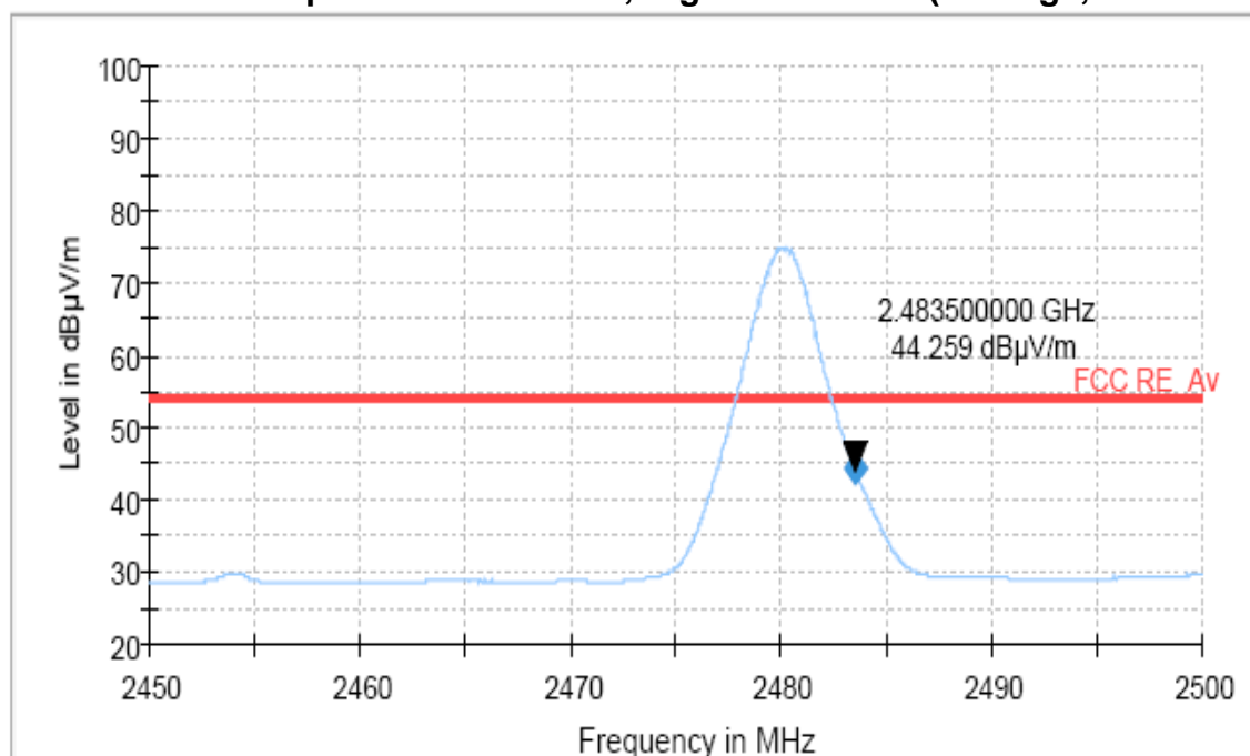
Restricted Band Spurious Emissions, Highest channel (Average, 8DPSK mode)
