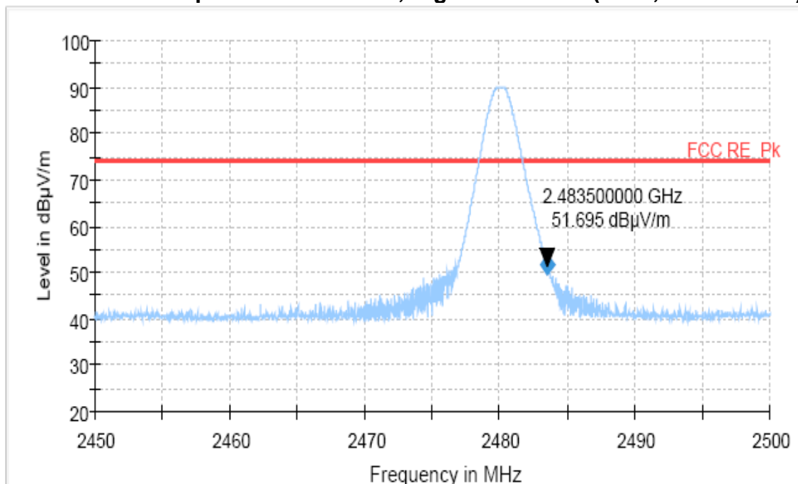
Restricted Band Spurious Emissions, Highest channel (Peak, GFSK mode)
