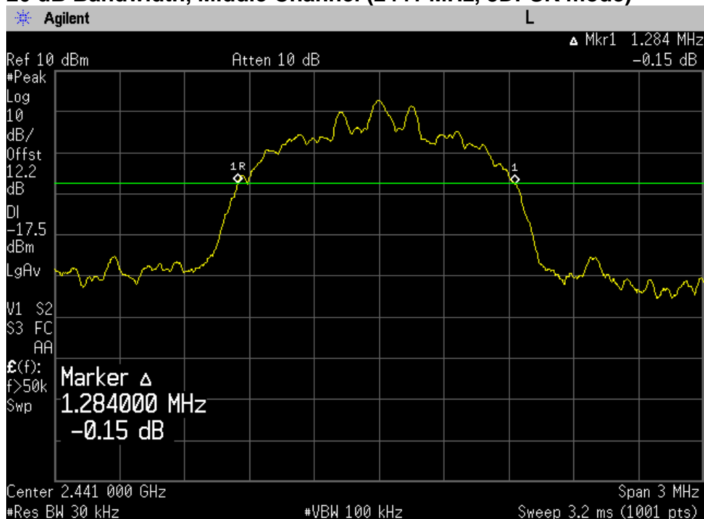
20 dB Bandwidth, Middle Channel (2441 MHz, 8DPSK mode)
