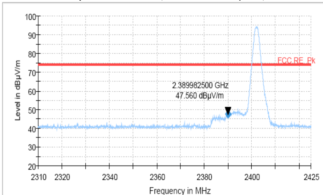
Restricted Band Spurious Emissions, Lowest channel (Peak, 8DPSK mode)
