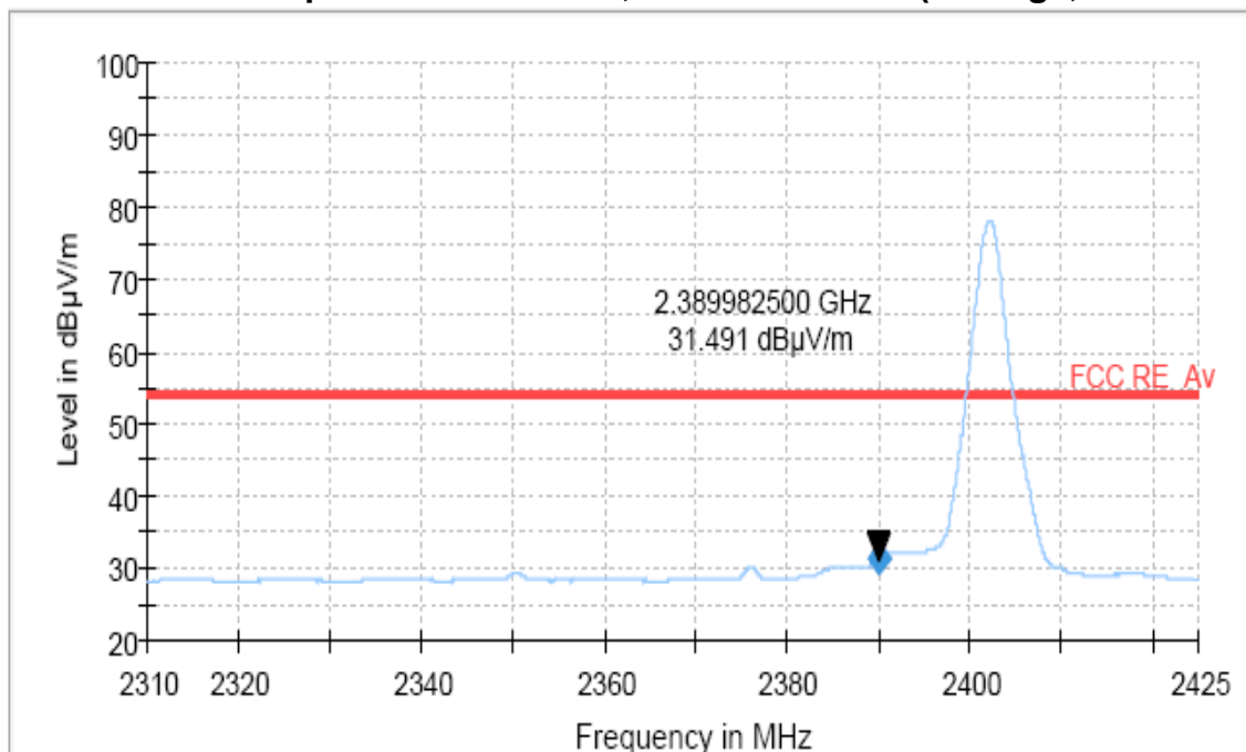
Restricted Band Spurious Emissions, Lowest channel (Average, 8DPSK mode)
