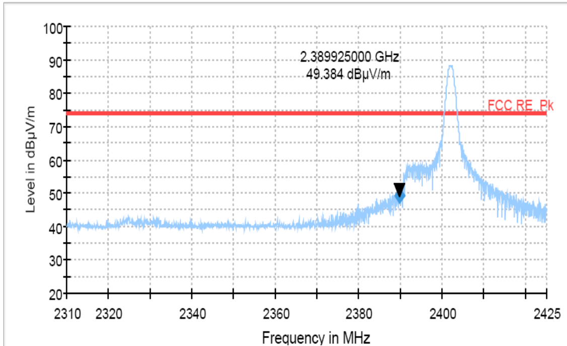
Restricted Band Spurious Emissions, Lowest channel(GFSK, Peak)
