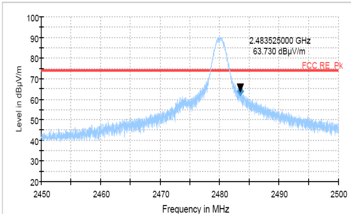
Restricted Band Spurious Emissions, Highest channel(GFSK, Peak)
