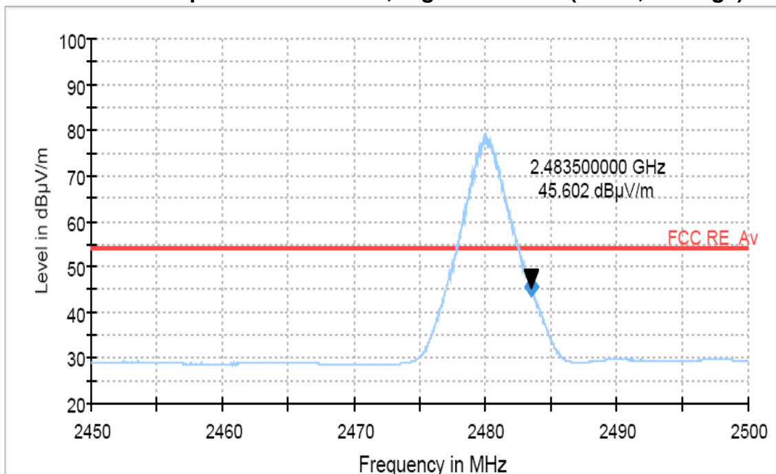
Restricted Band Spurious Emissions, Highest channel(GFSK, Average)
