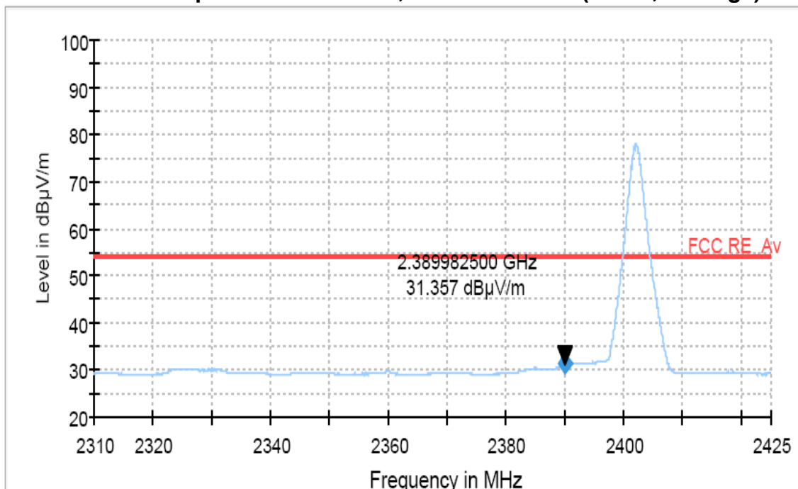
Restricted Band Spurious Emissions, Lowest channel(GFSK, Average)
