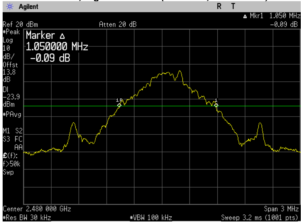
20 dB Bandwidth, Highest Channel (2480 MHz, GFSK Mode)
