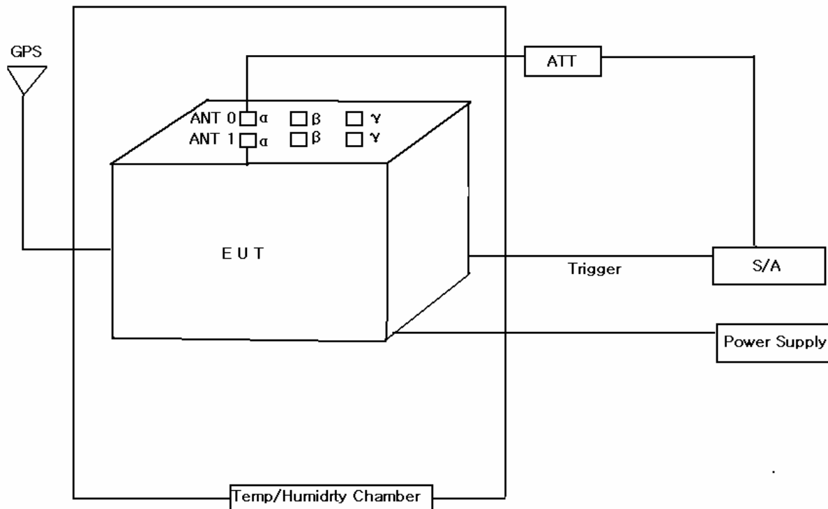
Conducted Test Setup
