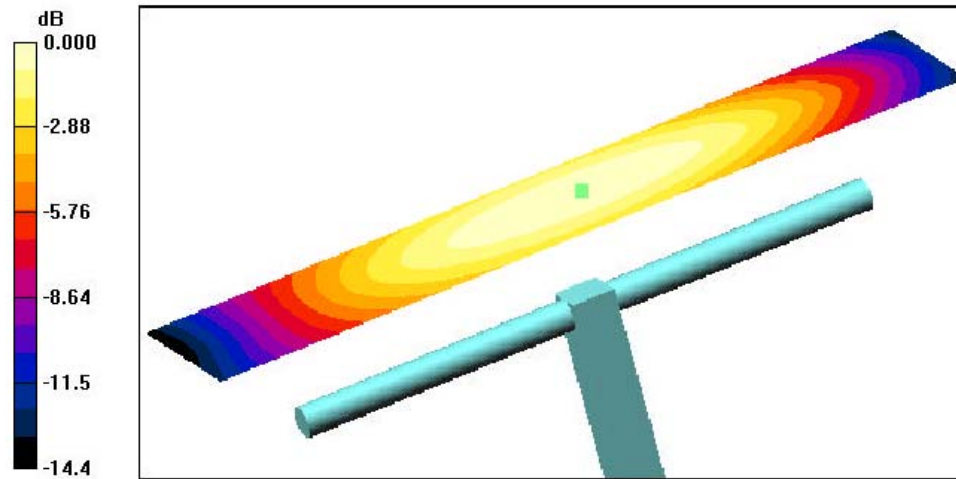
0 dB = 0.421A/m
