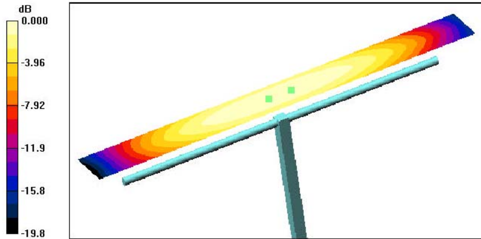
0 dB = 0.466A/m
