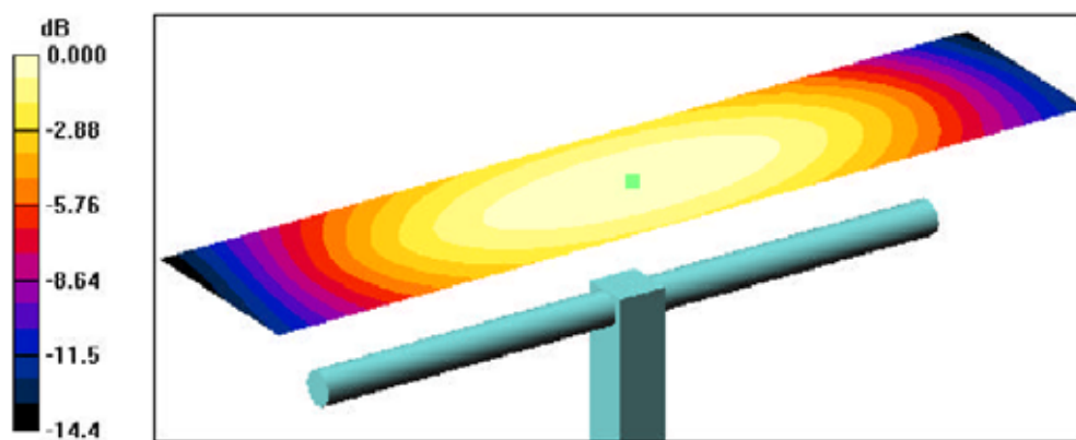
0 dB = 0.426A/m
