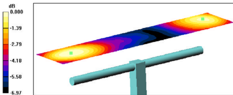
0 dB = 130.3V/m
