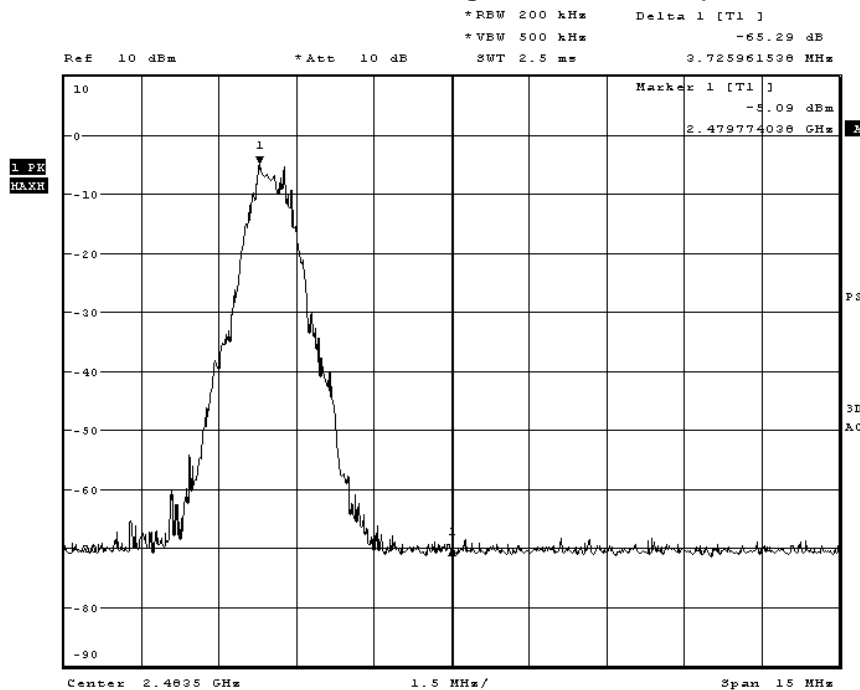
Plot 6-16 Measurement of Delta from Fundamental to Band Edge (Ch. 78)
