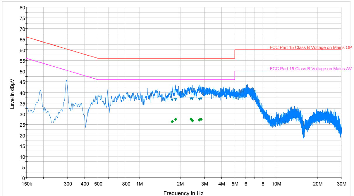
Plot 6-60. Line Conducted Plot with 802.11b (N)
