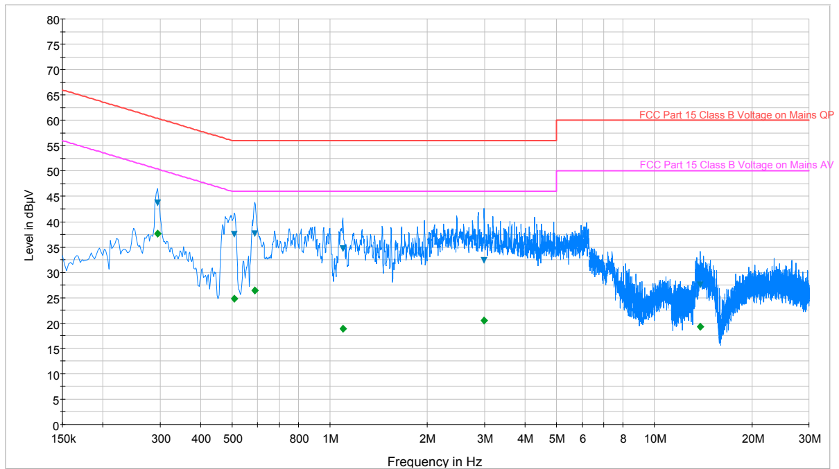
Plot 6-54. Line Conducted Plot with 802.11a UNII Band 1 (L1)
