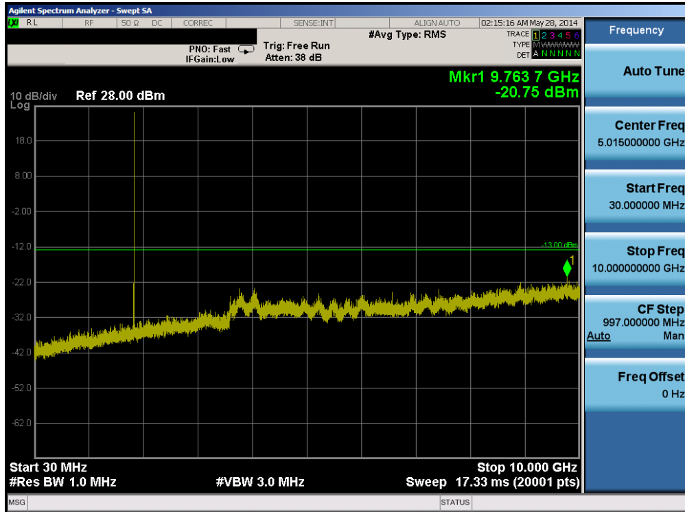
Plot 6-11. Conducted Spurious Plot (Band 25 – 3.0MHz QPSK – RB Size 1, RB Offset 0 – Low Channel)
