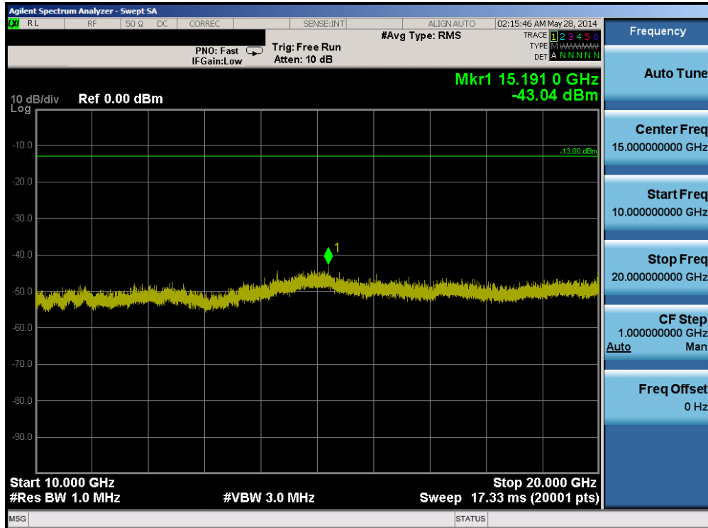
Plot 6-12. Conducted Spurious Plot (Band 25 – 3.0MHz QPSK – RB Size 1, RB Offset 0 – Low Channel)
