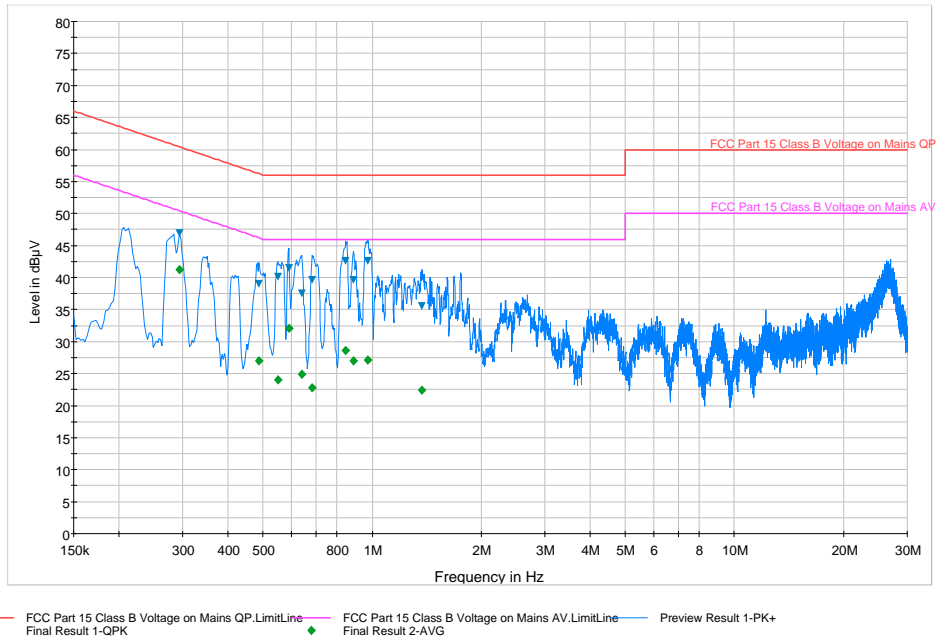
Plot 6-31. Line Conducted Plot with 802.11a (L1)
