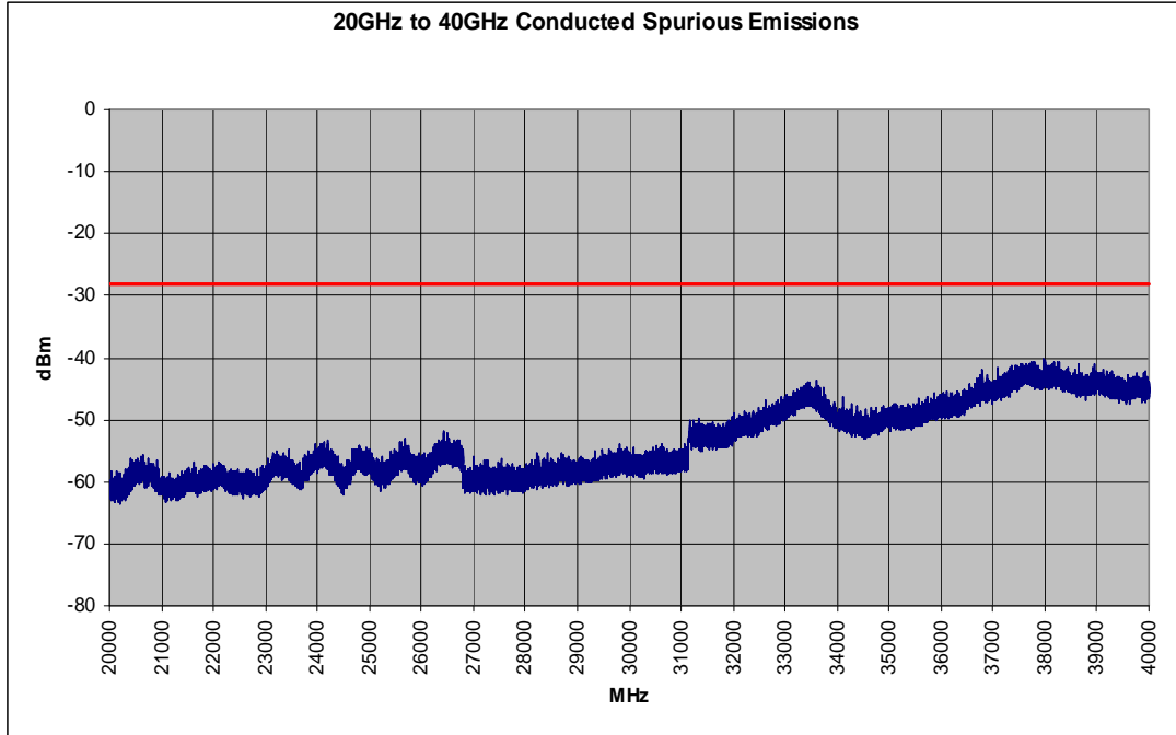
Plot 6-50. Conducted Spurious Plot (802.11a – Ch. 157)
