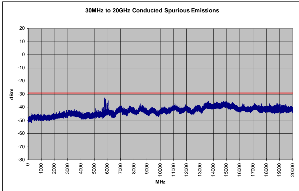
Plot 6-51. Conducted Spurious Plot (802.11a – Ch. 165)
