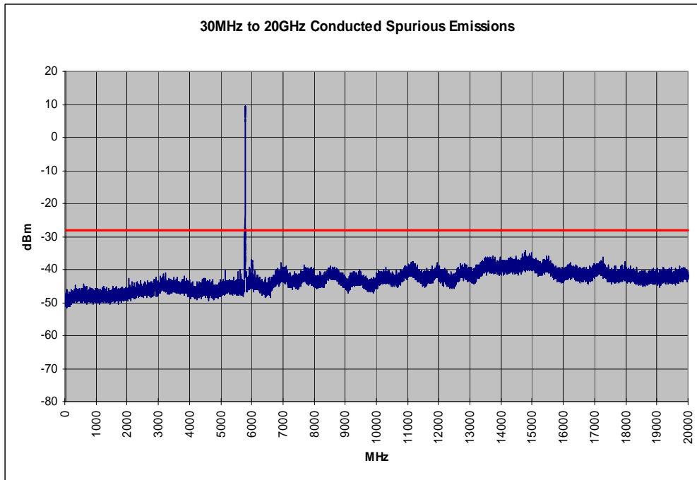
Plot 6-49. Conducted Spurious Plot (802.11a – Ch. 157)
