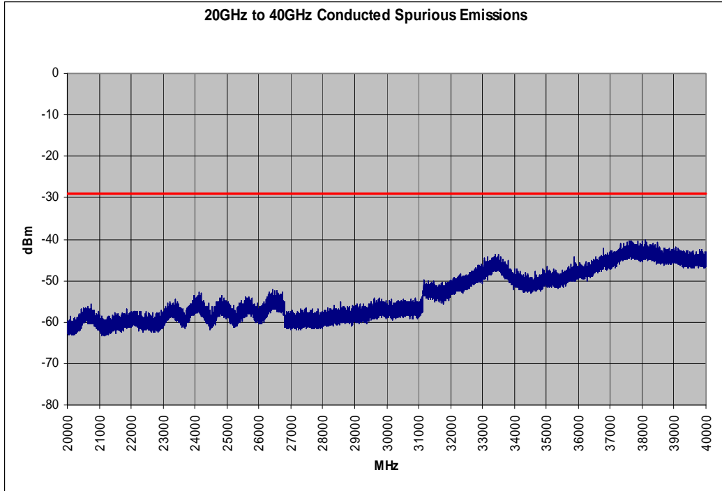
Plot 6-52. Conducted Spurious Plot (802.11a – Ch. 165)
