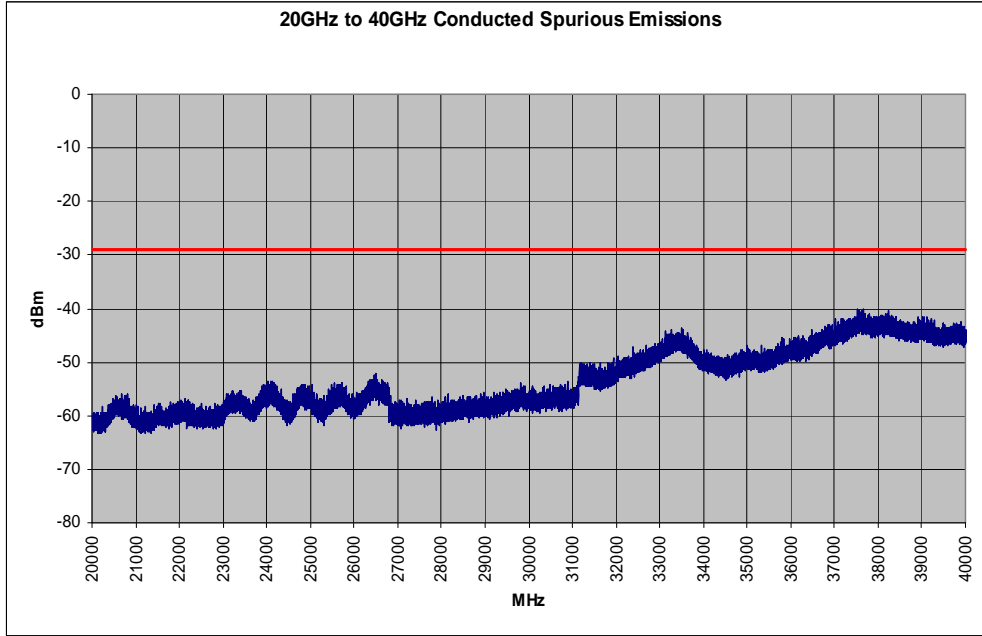
Plot 6-48. Conducted Spurious Plot (802.11a – Ch. 149)
