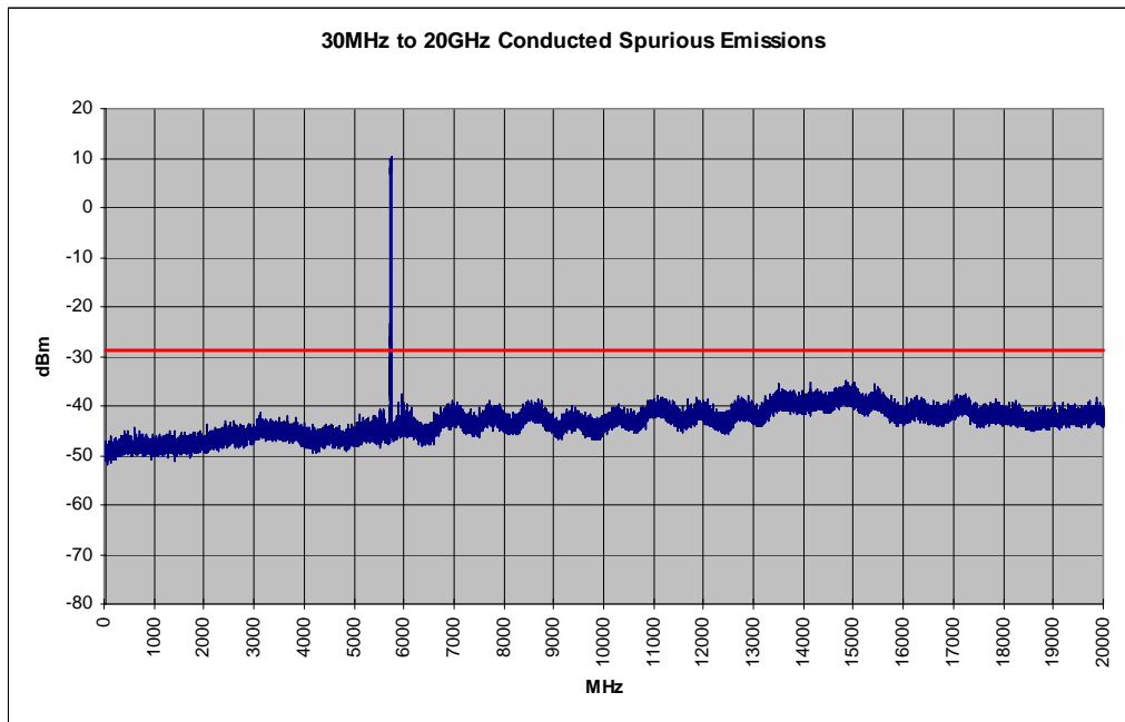
Plot 6-47. Conducted Spurious Plot (802.11a – Ch. 149)
