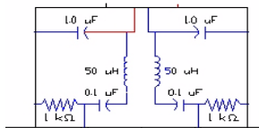
Figure 3-4. LISN Schematic Diagram
