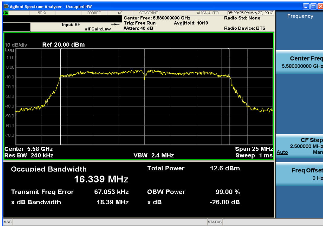
Plot 6-14. 26dB Bandwidth Plot (802.11a (UNII Band 3) – Ch. 116)
